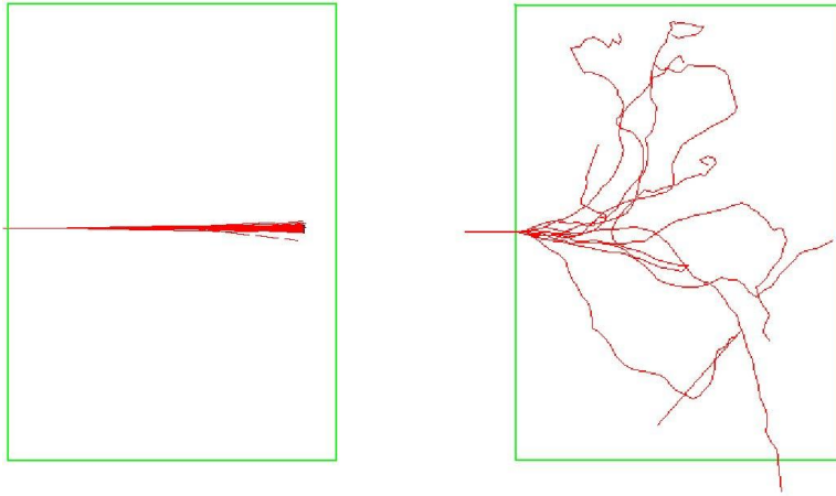
Figure 2.14 – Path of a magnesium ion, initial energy is 500 MeV (left) and of an electron, initial energy is 100 keV (right), inside a 500 \mu m silicon target
