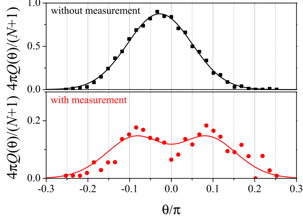
Figure 4.8: Tomography of quantum Zeno dynamics along trajectory I. High-resolution 1d cuts of the Husimi-Q distributions Q(\theta, \phi = 0) for t = 0.96 T without measurement (upper panel) and with a measurement with rate r_m \simeq 22\Omega (lower panel).
