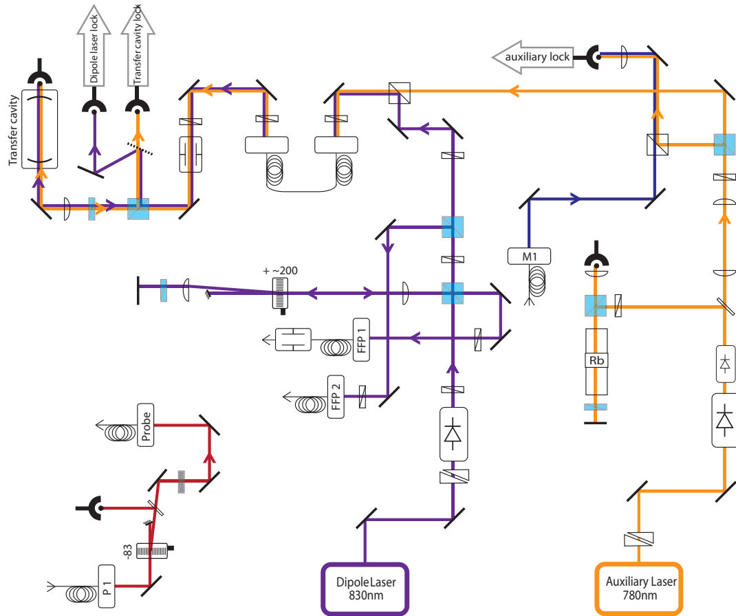
Figure 2.8: Beam paths on the “locking” table. For a legend of the symbols, see Figure 2.7. Adapted from [45].
