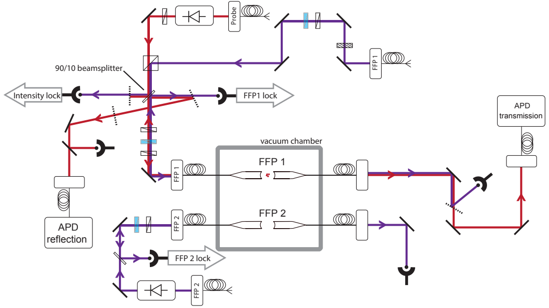
Figure 2.9: Beam paths on the “detection” table. For a legend of the symbols, see Figure 2.7. Adapted from [45].
