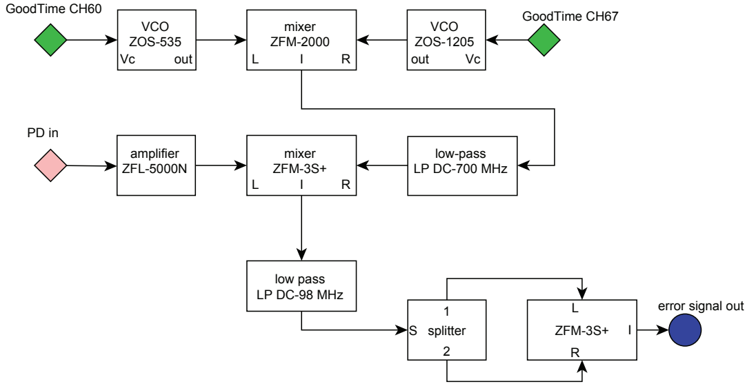
Figure B.1: Schematic of the RF electronics to generate the error signal between main and probe laser.
