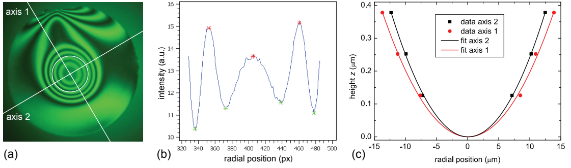
Figure 5.6: Determination of ROC using an interferometric measurement. (a): Interferometric microscope image of a microfabricated fibre facet ( \varnothing 125\mu\text{m} ). The white circle limits the region for the subsequent reconstruction. (b): Intensity cut of the image along axis 1. (c): Reconstructed profile cuts along the two axes. Parabola fits give R_1 = 250\mu\text{m} and R_2 = 210\mu\text{m} .
