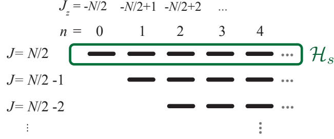
Figure 1.2: Structure of the angular momentum states |J, J_z\rangle for N two-level atoms. The subspace \mathcal{H}_s of fully symmetric states is spanned by the Dicke states \{|n_N\rangle \equiv |J = N/2, J_z = -N/2 + n\rangle\} .
