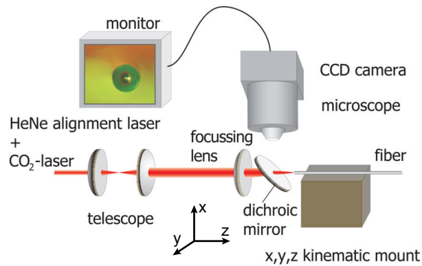
Figure 5.1: Schematic of the \text{CO}_2 laser setup used to micro-fabricate the fibres for the FFP experiment. Adapted from [63].
