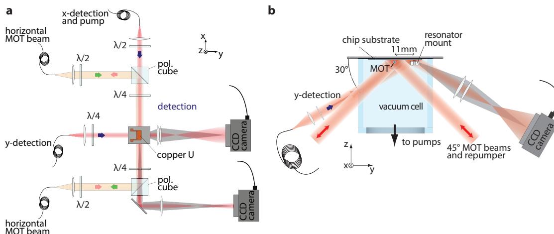
Figure 2.10: Schematic of the optics surrounding the vacuum cell. a) Top view showing in particular the two horizontal MOT beams. b) Side view. The position of the mirror-MOT is constrained by the condition that the resonator bridge should not clip the 45° beams. y-detection is used for absorption imaging of the MOT region, x-detection of the resonator region. Adapted from [63].
