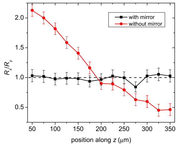
Figure 5.3: Ratio of horizontal to vertical radius of curvature R_x/R_y of \text{CO}_2 laser-machined structures (waist size about 32 μm). The dichroic mirror used for alignment produces astigmatism so that the symmetry of the structures varies with the position on the beam axis z .
