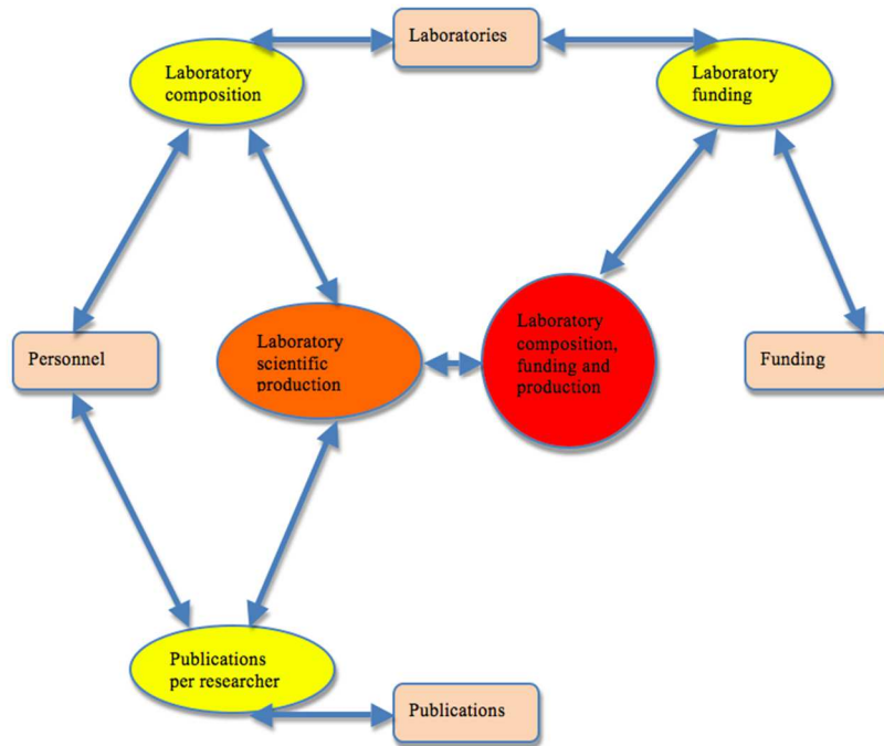
Figure 10 Data structure
