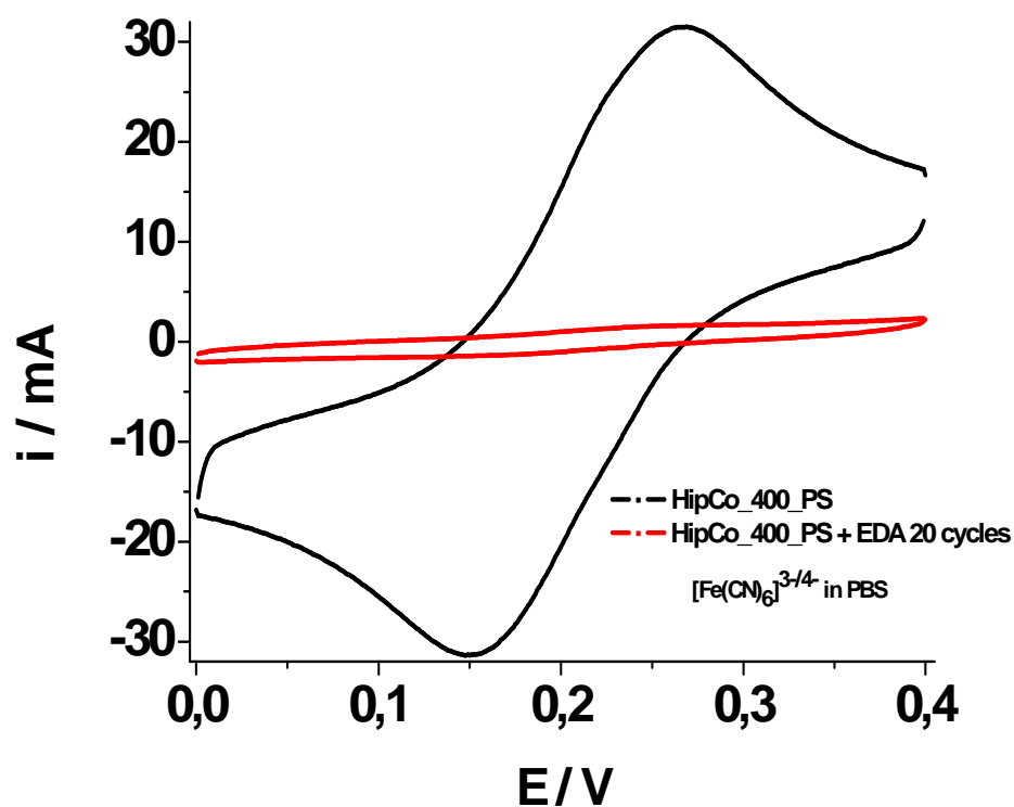
Fig. 4a: Cyclic voltammetry of \text{K}_3[\text{Fe}(\text{CN})_6]^{3-/4-} at the electrode surface before (black line) and after (red line) electrochemical modification with 5 mM EDA in PBS; scan rate 100 \text{ mV s}^{-1}
