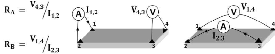
Fig. 4: Schematic representation of a Van der Pauw configuration used in the determination of the two characteristic resistances R_A and R_B .
