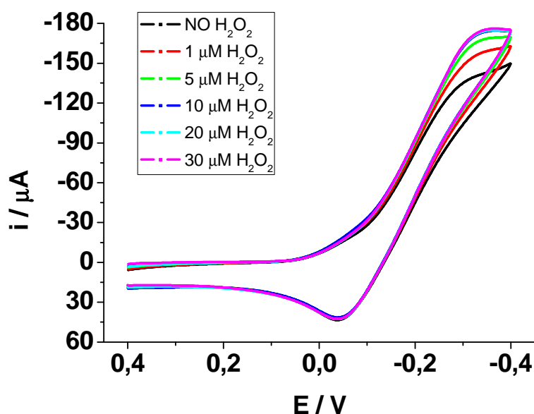
Fig. 14a: Cyclic voltammetry for the electron transfer of the redox shuttle HQ \rightleftharpoons BQ (1 mM Hydroquinone in PBS) at the SWCNT-modified electrode upon an increasing concentration of hydrogen peroxide. Reference electrode was Ag/AgCl.
