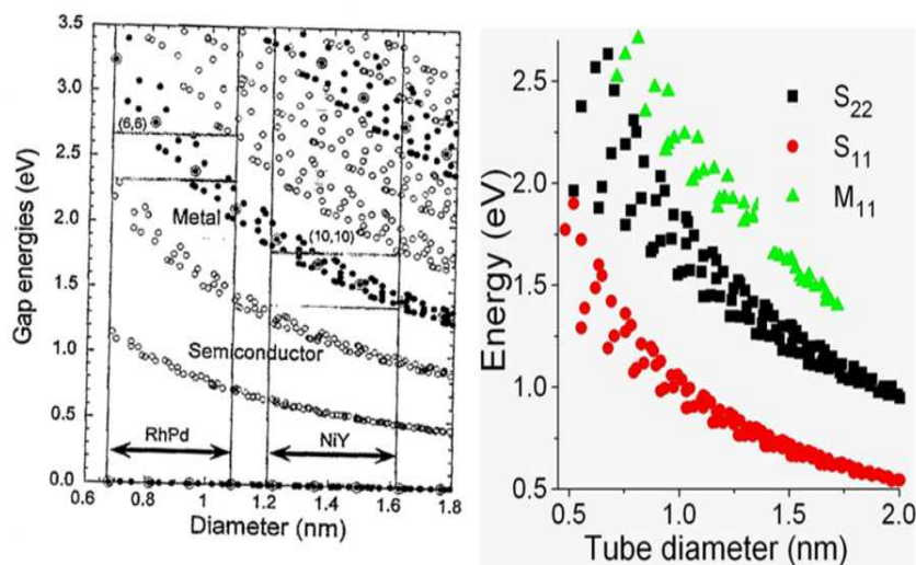
Fig. 3: Kataura's plot showing specific resonant nanotubes (metallic or semiconducting) when excited at specific laser energy. From: Optical properties of single-walled carbon nanotubes. 6
