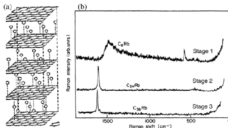
Fig. 9: GIC representation (left) and Raman spectra (right) obtained for different stage index GICs in 1970s. From: Physica scripta, 2012. 29
