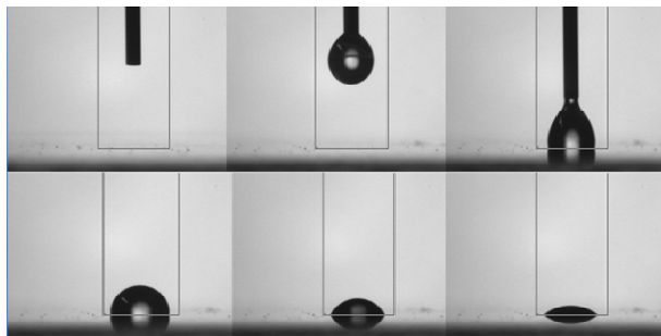
Fig. 8: Contact angle measurement of a SWCNT film deposited on glass.
