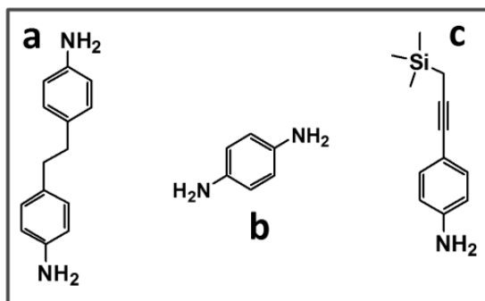
Fig.2: Aryl-amines selected for the electrochemical surface modification of SWCNT based electrodes. (a) 4, 4'- Ethylene dianiline (EDA), (b) p-Phenylenediamine (p-PhDA)., and (c) 4-[(Trimethylsilyl) ethynyl] aniline (TMS).
