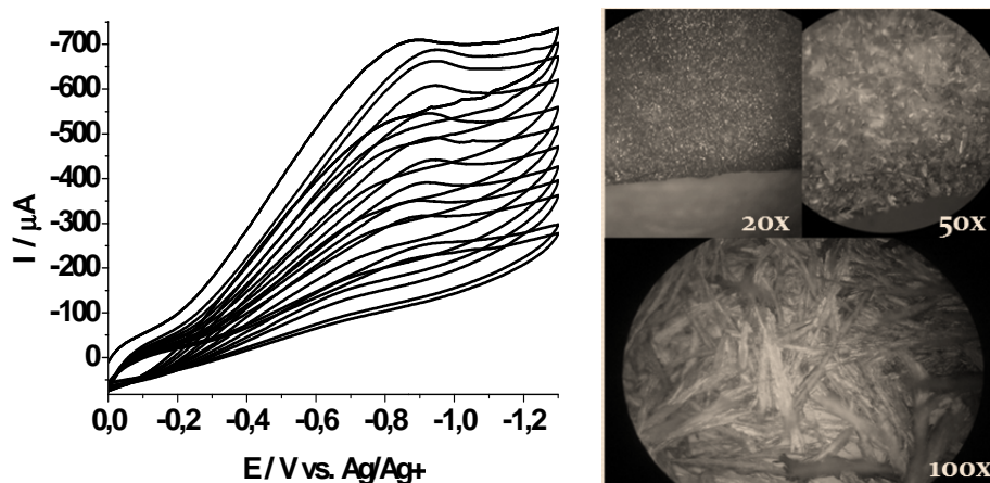
Fig. 17: Cyclic voltammetry for the electrochemical surface modification of CoMoCAT SWCNT based electrode with 10 mM solution of BDT in acetonitrile. Scan rate: 50 \text{ mV s}^{-1} . Optical images for the resulting crystalline film formed during the process at different magnifications.
