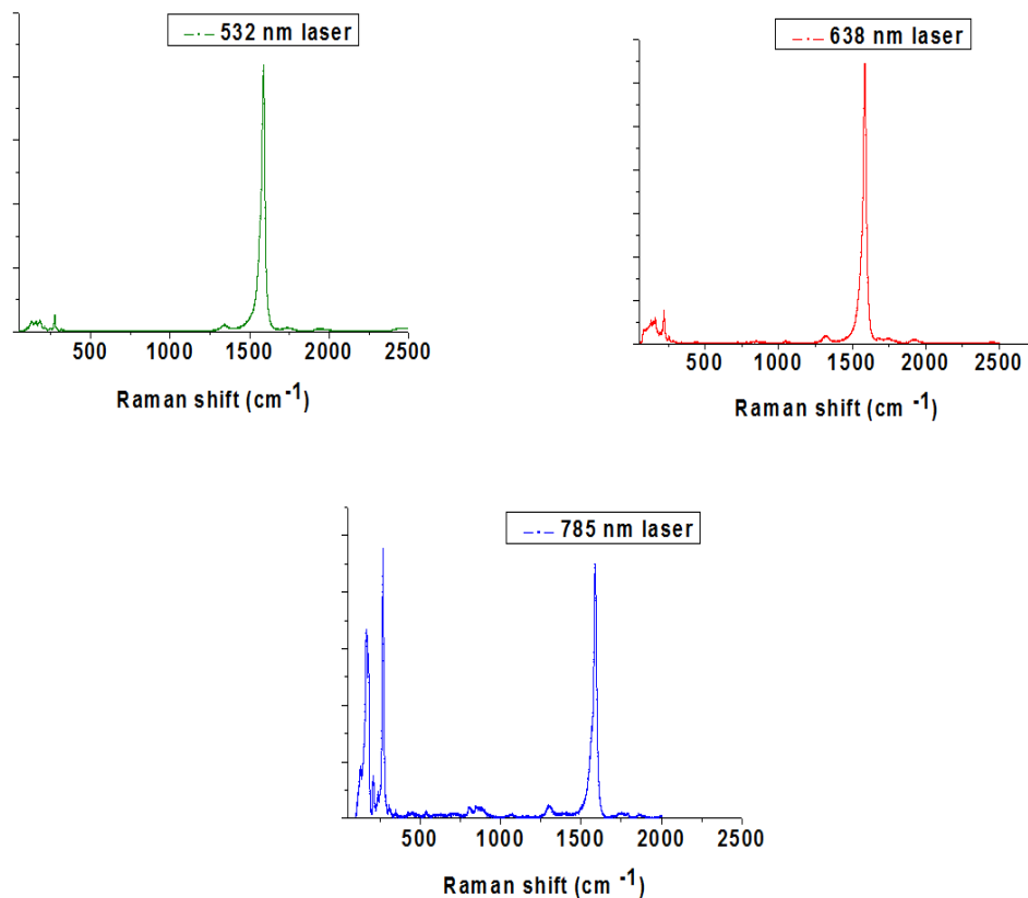
Fig. 10: Raman spectra of Rice-SWCNT film on silanized glass measured at three different excitation lasers.
