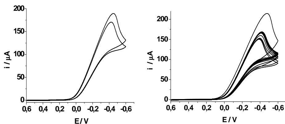
Fig. 13: Cyclic voltammetry for the electrochemical surface modification of graphene film with 5 mM 1, 3- BDYT in acetonitrile. Left: 2 cycles. Right: 20 cycles. Scan rate: 50 \text{ mV s}^{-1} .
