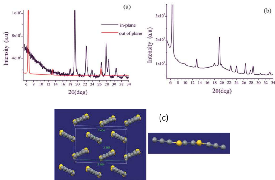
Fig. 26b: (a) Diffraction patterns of evaporated DB-TTF film, (b) Out-of-plane diffraction patterns of DB-TTF film prepared by dropcasting (the \lambda used was 0.154 nm), and (c) crystal structure of the \beta -phase of DB-TTF along the molecular axis. Sulfur atoms are identified in yellow. 102
