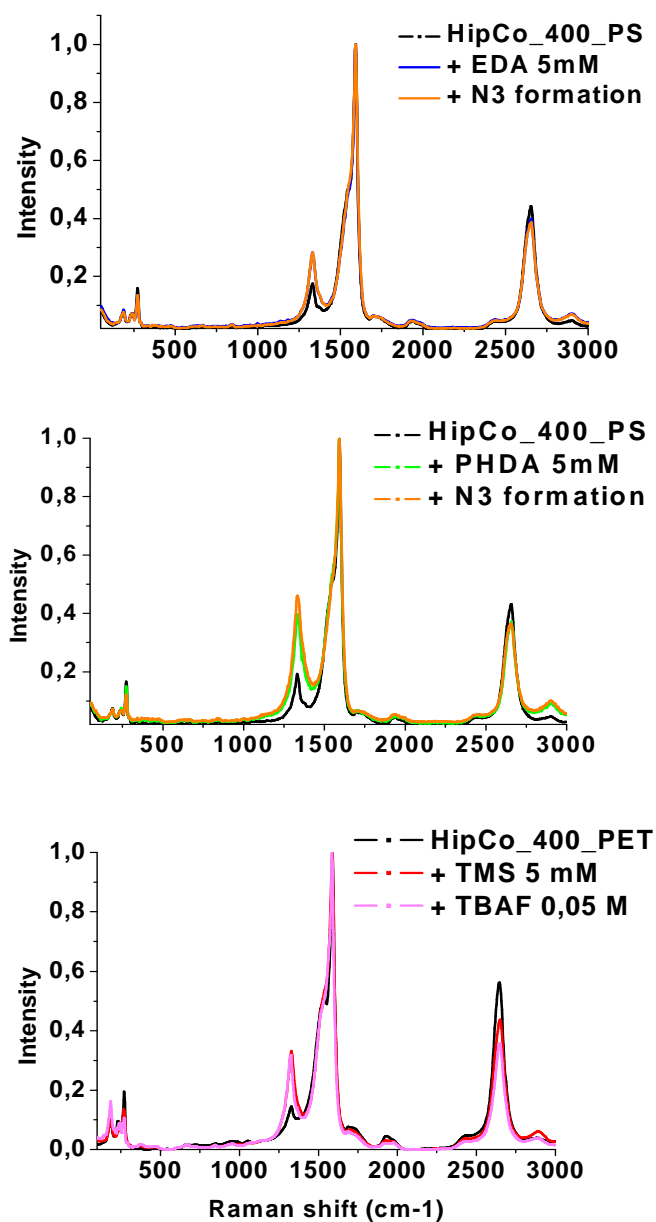
Fig. 8: Raman spectra of SWCNT films after chemical transformation of modified surfaces for the three different approaches (EDA, PhDA, and TMS molecules). Excitation laser used was 532 nm for the three measurements.
