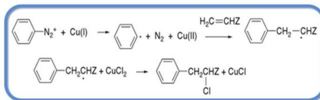
Fig. 10: Arylation reaction: Meerwein Arylation.
