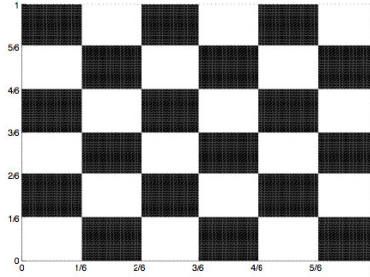
Figure 4.4: Checker-board function.
