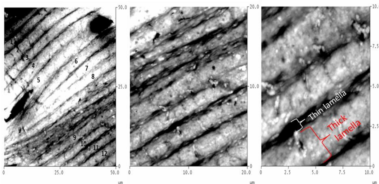
Figure 3.12 Contact mode height AFM images of the interstitial lamellae of the rat cortical shell. The scan rate was \sim 3.0 Hz and the z-scale=150 nm.
