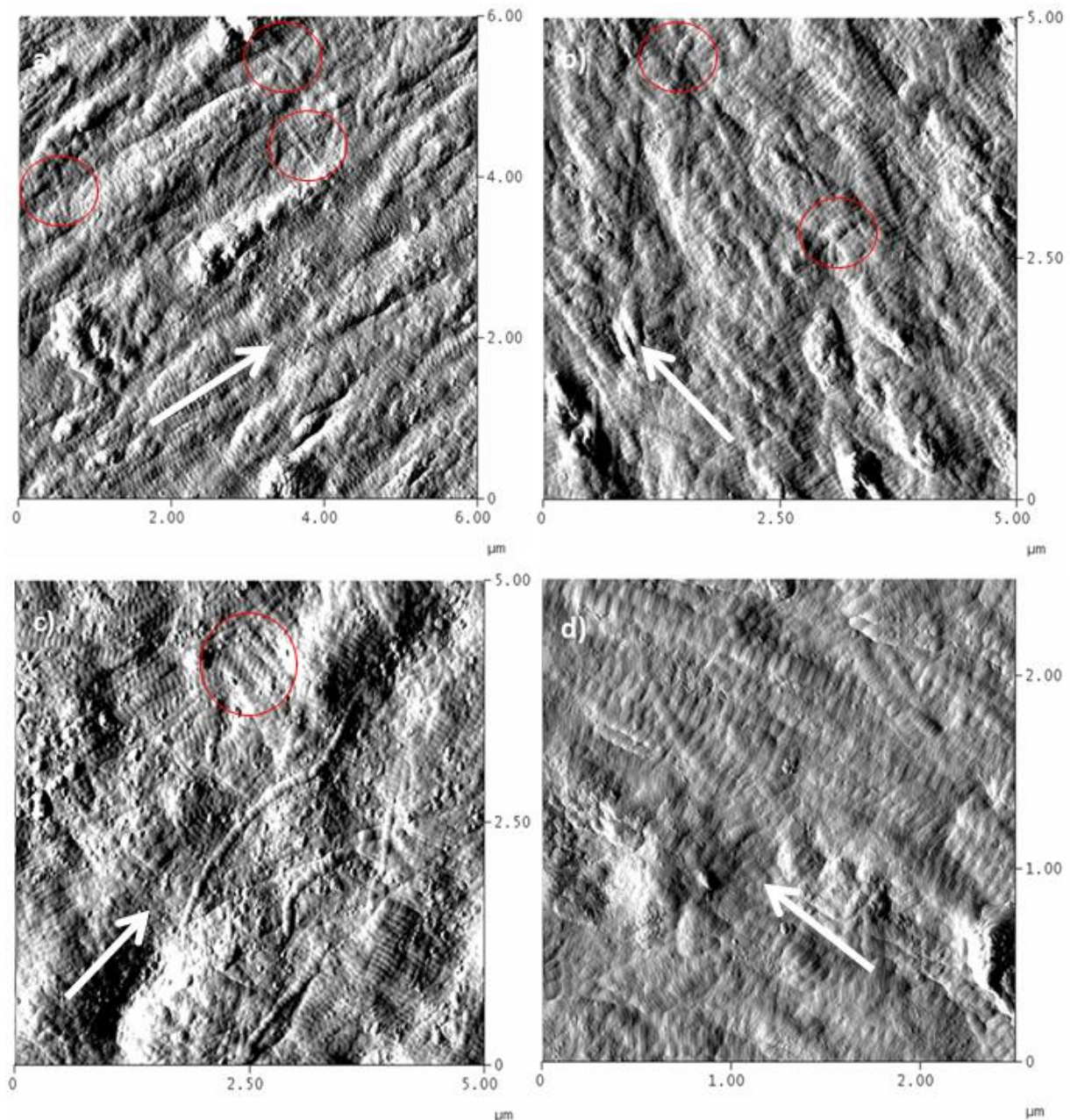
Figure 3.14 Mineralized collagen fibrils obtained by a), b) and d) Contact mode deflection AFM image scan rate \sim 1.8 Hz and data scale 18 mV c) Tapping mode amplitude AFM image, scan rate \sim 1.8 Hz and data scale 650 mV. The arrows suggest a possible privileged direction for fibrils orientation and the circles signal isolated collagen fibrils that cross the privileged orientation.
