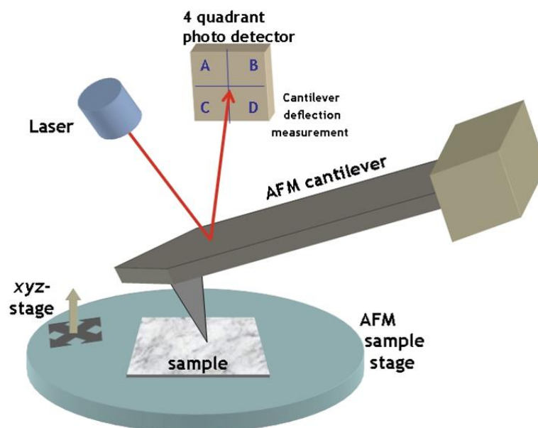
Figure 1.18 Typical atomic force microscope (AFM) setup: The deflection of a micro fabricated cantilever with a sharp tip is measured by reflecting a laser beam off the backside of the cantilever while it is scanning over the surface of the sample. (Open source Handbook of Nanoscience and Nanotechnology)
