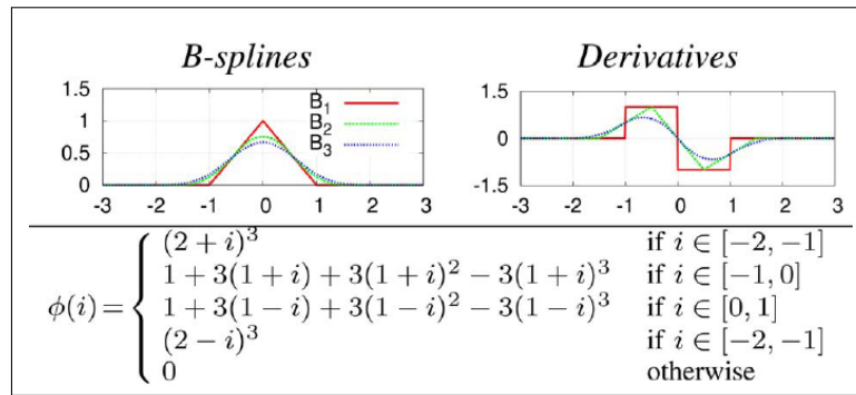
Figure 1.9 – B-spline functions used in MI based Visual Servoing [Dame 10]
