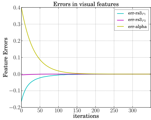
(b) WPM - Errors in rs_{3p1}, rs_{3p2}, \alpha
