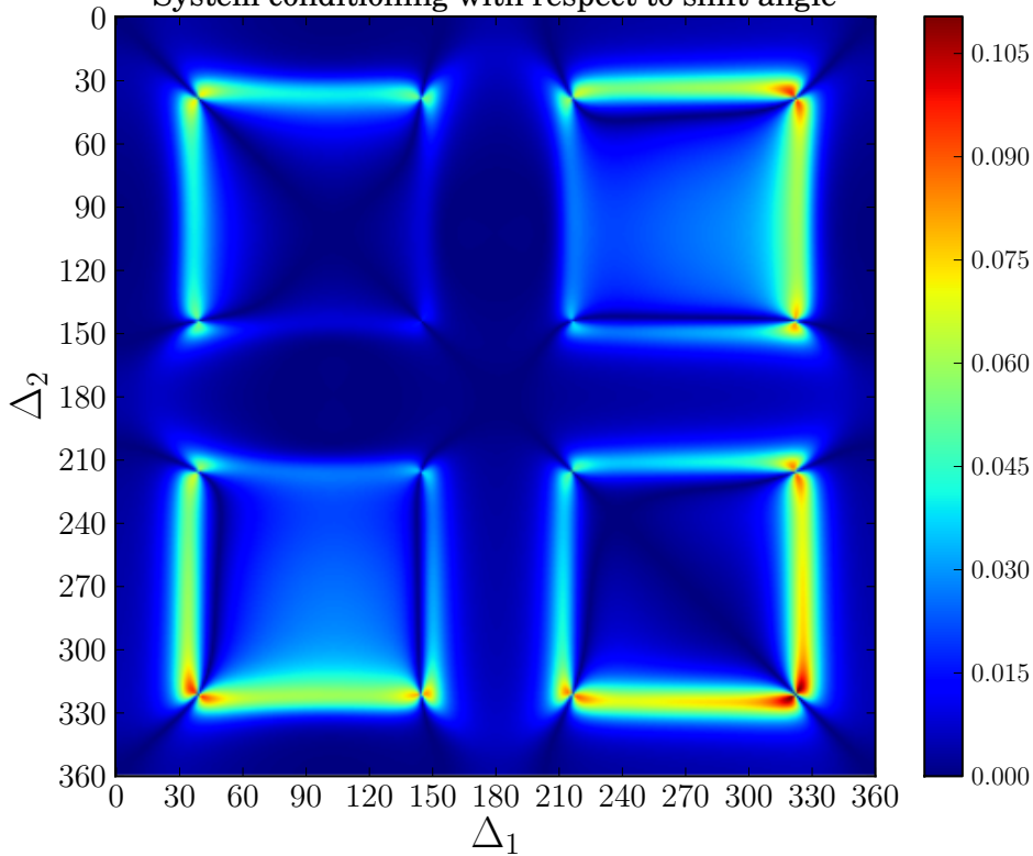
(c) Joint selection of \Delta_1 and \Delta_2
