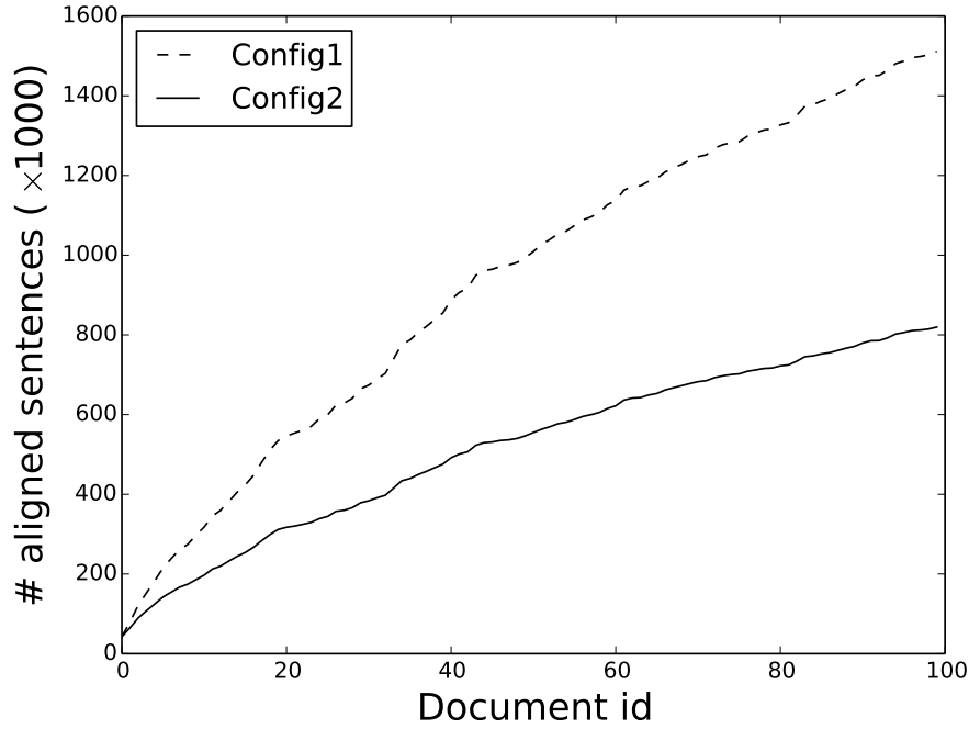
Figure 4.2: Evolution of the cache size for a sequence of Cochrane documents.
