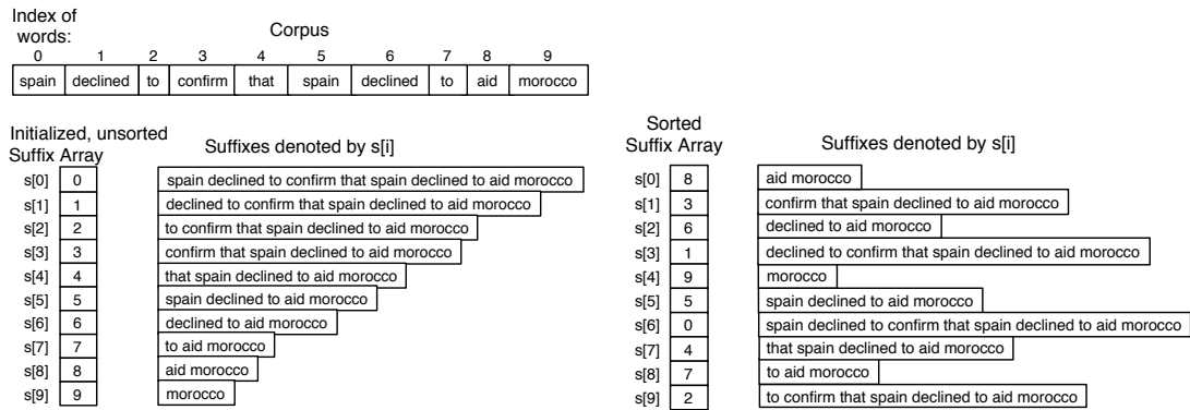
Figure 2.1: Illustration of suffix array for a very small corpus (reproduced from [Callison-Burch et al., 2005]).
