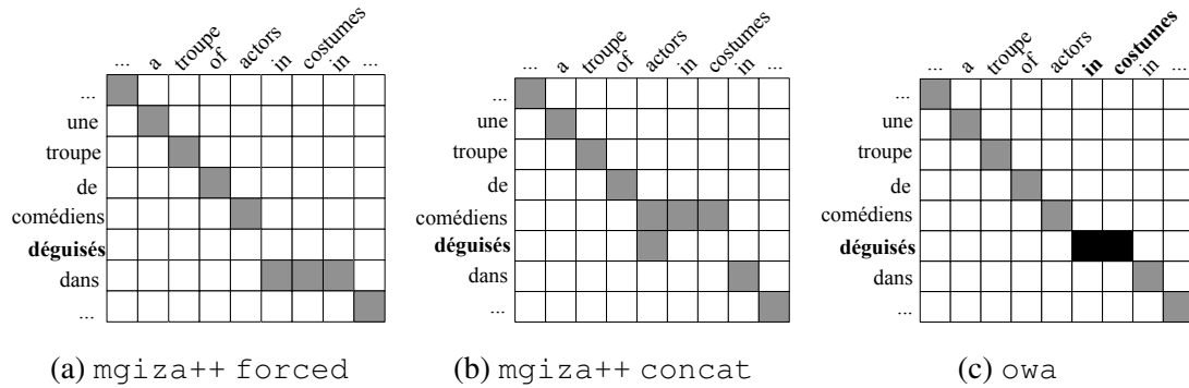
Figure 3.7: Example of matrices on French-English obtained using two mgiza++ baselines and our on-demand word alignment ( owa ).
