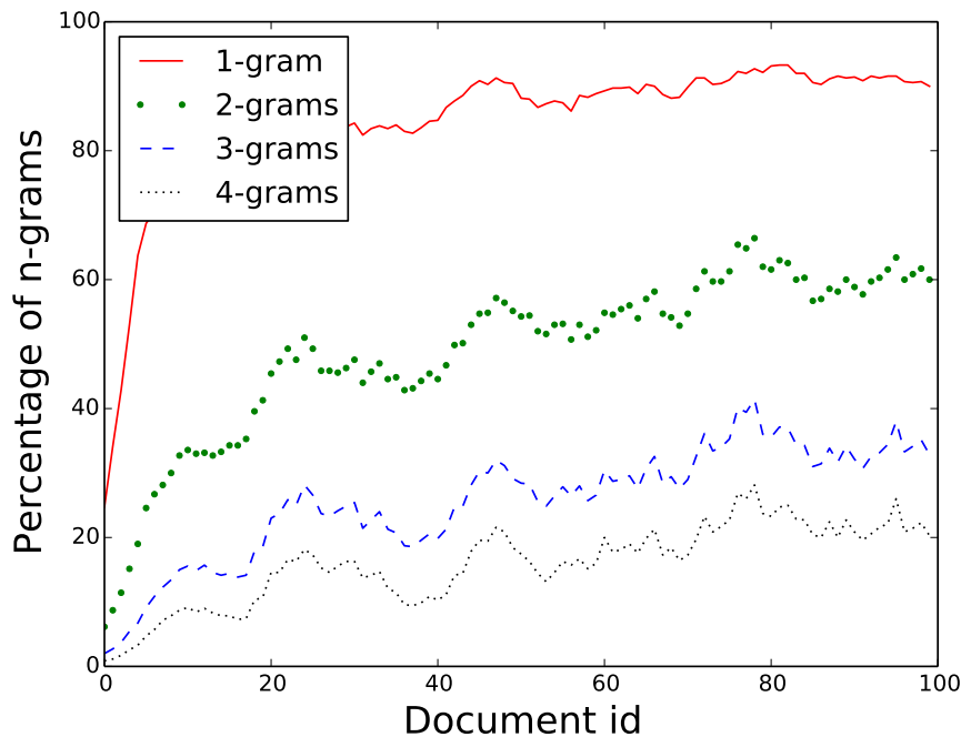
Figure 4.1: Percentage of n -grams found in previous documents in the Cochrane document sequence.
