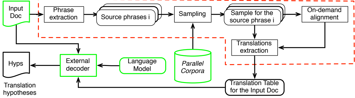
Figure 3.6: Main processes of our framework (delimited by a red frame).
