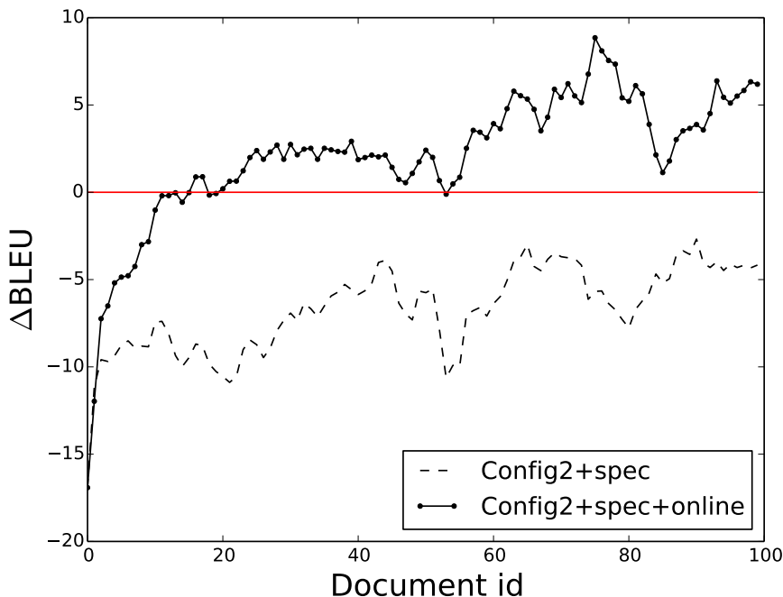
Figure 4.6: Document-level comparison with the vanilla moses system with online tuning. Initialization either uses moses default values ( +spec+online ), or parameters tuned on a development set ( +dev ).
