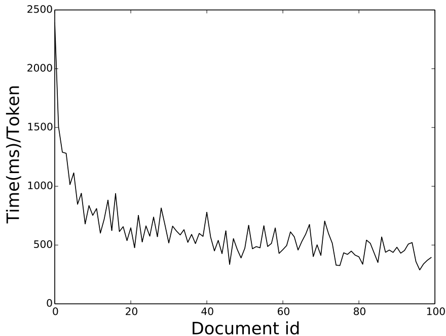
Figure 4.3: Evolution of the average per token processing time for a sequence of documents.
