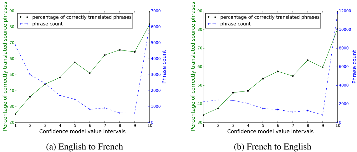
Figure 5.1: Percentage of correctly translated source phrases in the trace of the decoder of the TF-IDF+conf systems against score value intervals of the confidence model (conf) in the Newstest translation task. The dashed line represents the number of phrases in each confidence value interval.
