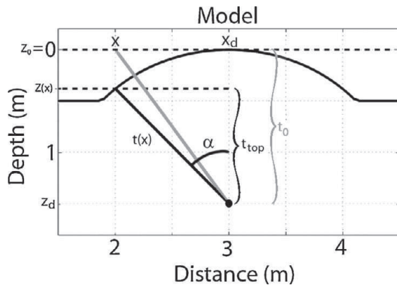
Fig. 2. Schematic presentation showing the topographic correction for the Kirchhoff migration. For a given position x at the surface z_0 = 0 , we take into account the topography z(x) instead of considering the flat datum plane (dashed line at z_0 = 0 ). The travel time t(x) is now calculated along the thick line path rather than along the grey line one.
