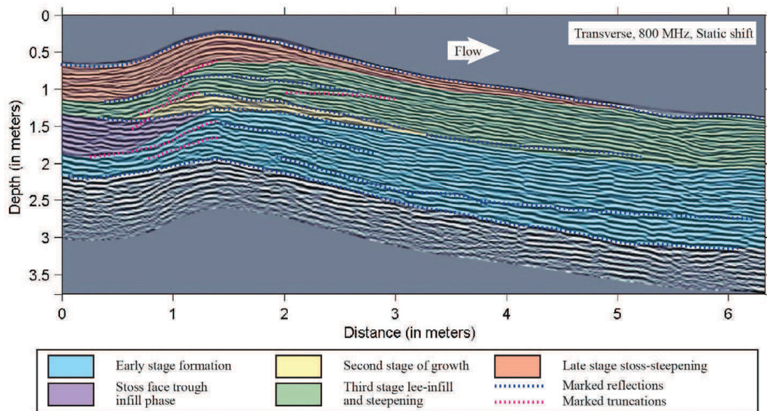
Figure 12 : Representative profile with the 800 MHz antenna over a transverse dune bedform from Achupashal ash body III. Main reflections and interpreted units are highlighted, see legend. The base unit, not highlighted, is interpreted as the possible pre-eruptive soil.
