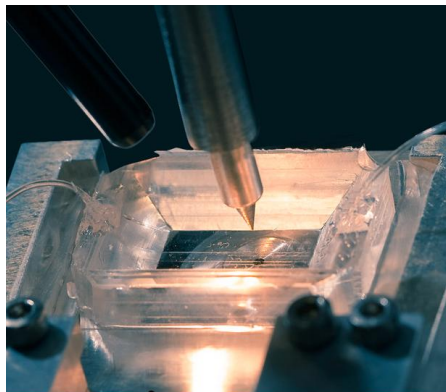
Figure 64: Adapted from [143]. On the left, photography of the FRMT experimental setup; illumination is achieved by the use of an optical fiber (top left on the photo). On the right, photography of the magnetic tip coupled with two LED to achieve better homogeneous illumination.
