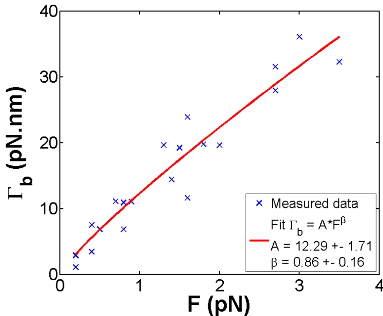
Figure 113: Buckling torque \Gamma_b as a function of the magnetic pulling force F (blue data points). The measured data is fitted with a power law (red profile) showing a dependency to the force with a power coefficient \beta=0.86 .
