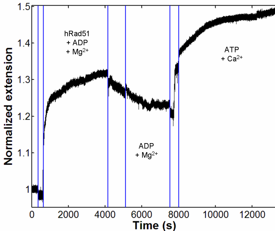
Figure 138: Experiment showing nucleotide turnover in a filament formed on a nicked dsDNA molecule. Around t \approx 350 s, a buffer containing 200nM hRad51, 1mM ADP, 2mM MgCl_2 , 1mM DTT, 0.05% Tween 20, and 25mM NaCl was introduced in the chamber. A partially stretched filament was formed with a stretching of \sim 30\% . Free proteins in solution were then chased by the same buffer without hRad51 ( t \approx 4150 s). The molecule's extension decreases to a stretching of \sim 25\% . After some time ( t \approx 7525 s), a buffer containing 1mM ATP, 2mM CaCl_2 , 1mM DTT, 0.05% Tween 20, and 25mM NaCl was injected in the chamber. The molecule's extension reaches \sim 1.5 times its initial length, a fully stretched filament was formed. During the experiment, a pulling force of F = 7.96 pN was maintained.
