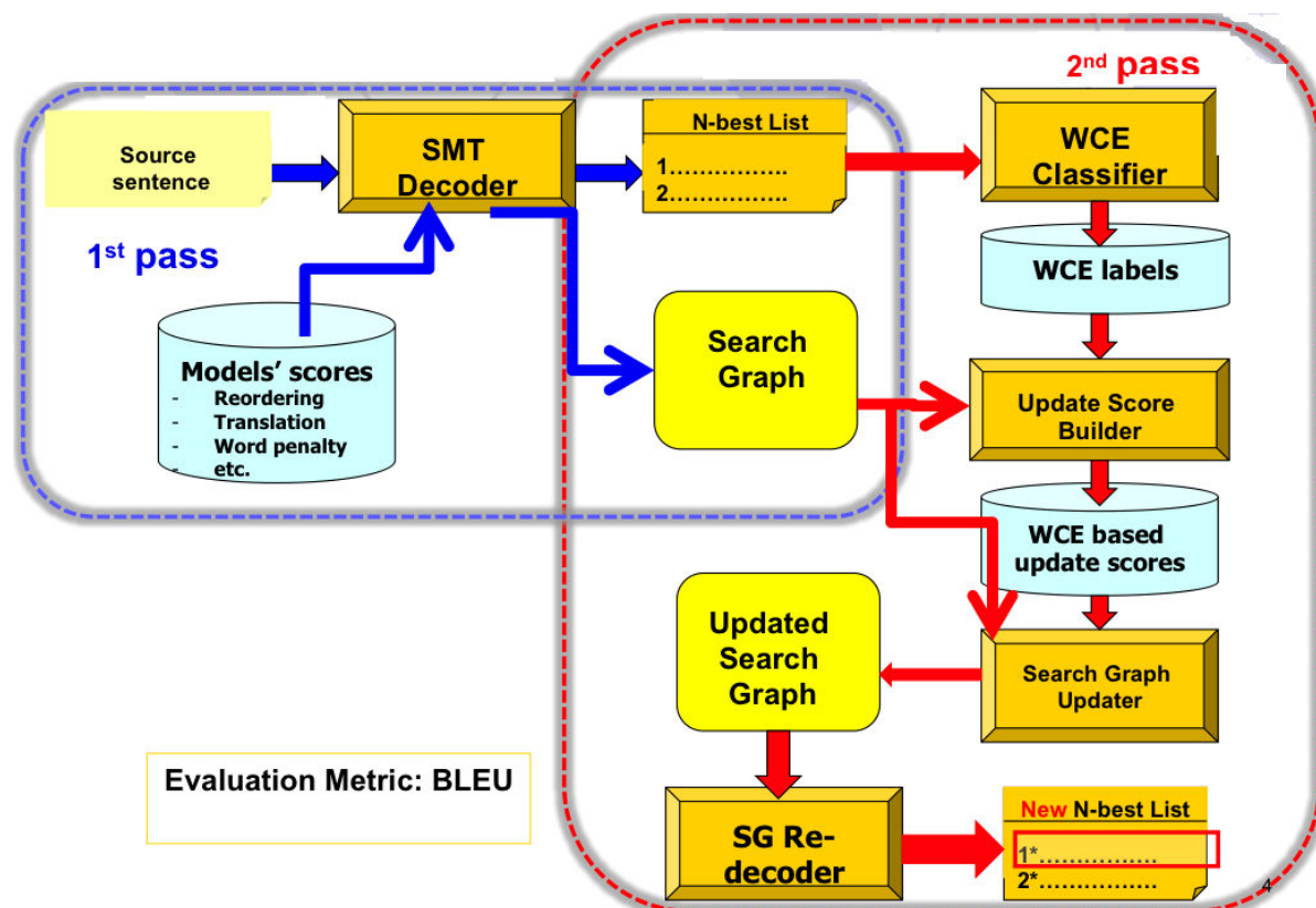
Figure 7.2 – Re-decoding Process
