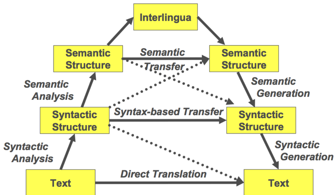
Figure 1.1 – Vauquois’s triangle
