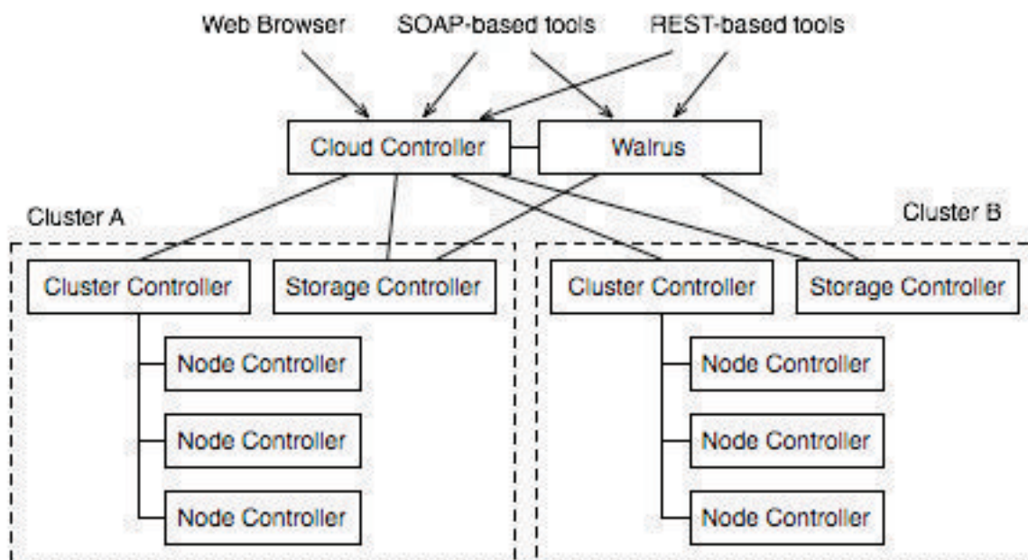
FIGURE 3.2 – Architecture de l'outil Eucalyptus
