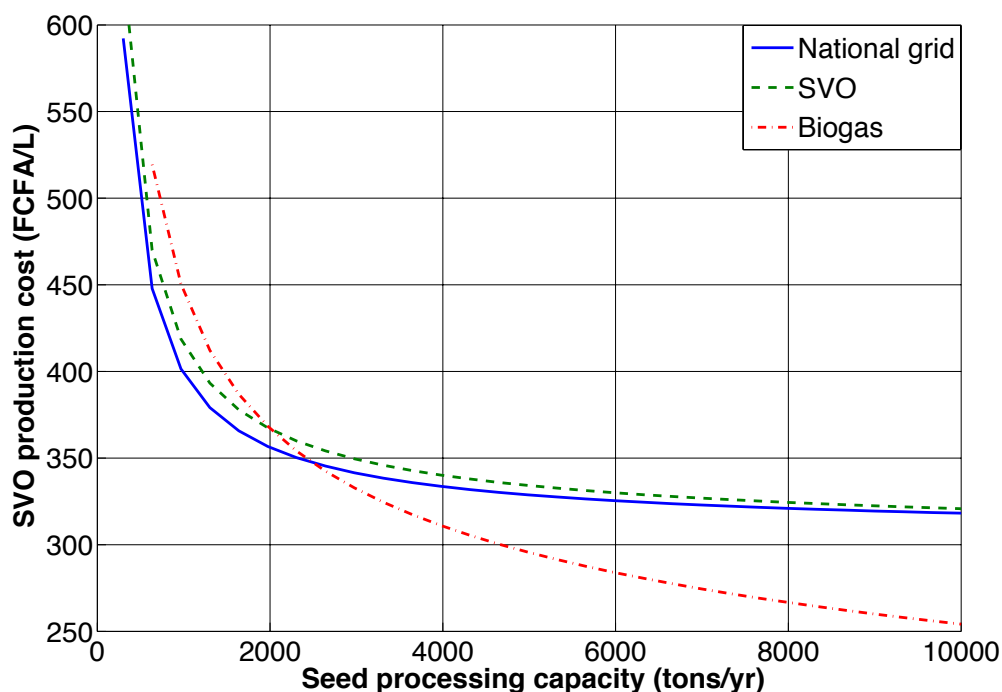
Figure 37. SVO production cost with respect to seed processing capacity and energy supply option.
