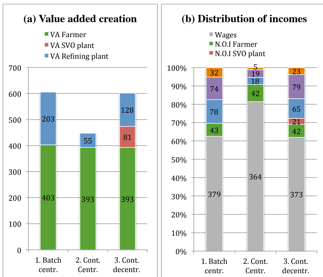
Figure 52. a) Value added creation by farmers (VA Farmer), SVO plant (incl. VAT) (VA SVO plant) and refining plant (incl.VAT) (VA Refining plant). b) Distribution of this value added in the form of incomes to employees (wages), to supply chain players (net operating incomes (N.O.I.) of farmers, SVO and refining plants), to the state (Taxes, including VAT) and to the banks (Financial costs). This is declined for the three refined oil supply chains. Figures in charts indicate the VA in FCFA/L of refined oil (see Chapter 2, Section 3.3).
