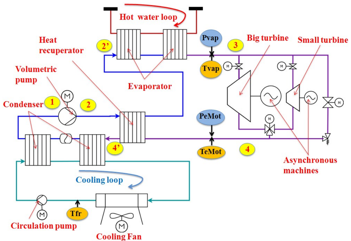
Figure 7.2: Schematic of the Organic Rankine Cycle Power Plant.
