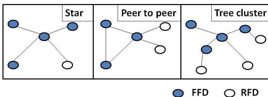
Figure 2.2: Three ZigBee topologies
