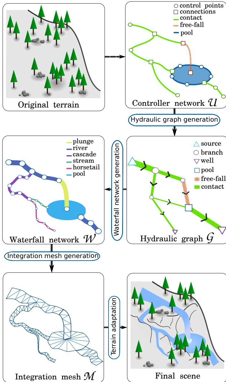
Figure 4.4: Processing pipeline used for creating waterfall scenes. The first step is the creation by the artist of the controller network \mathcal{U} . Then, a hydraulic graph \mathcal{G} is generated; the width of an arc encodes flow quantity. The waterfall network \mathcal{W} is then generated with a subdivision algorithm, and the waterfall types are determined. Finally, the integration mesh \mathcal{M} is generated. It is used to deform the terrain and to generate procedural details.
