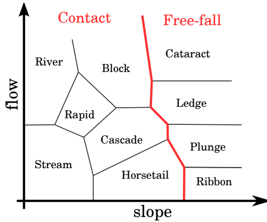
Figure 4.3: Our classification of waterfall types.
