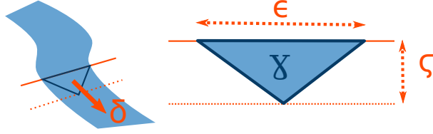
Figure 4.8: Triangular cross section of a waterfall segment, with a constant flow.
