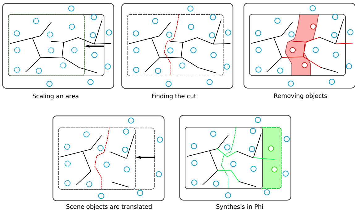
Figure 6.14: Shrinking a region: the user drags the region contour to shrink it. The algorithm finds the best cut in the scene. The objects in the cut region are removed. The objects are translated on the scene depending on the cut size and scaling direction. New objects are synthesized in the empty space at the right.
