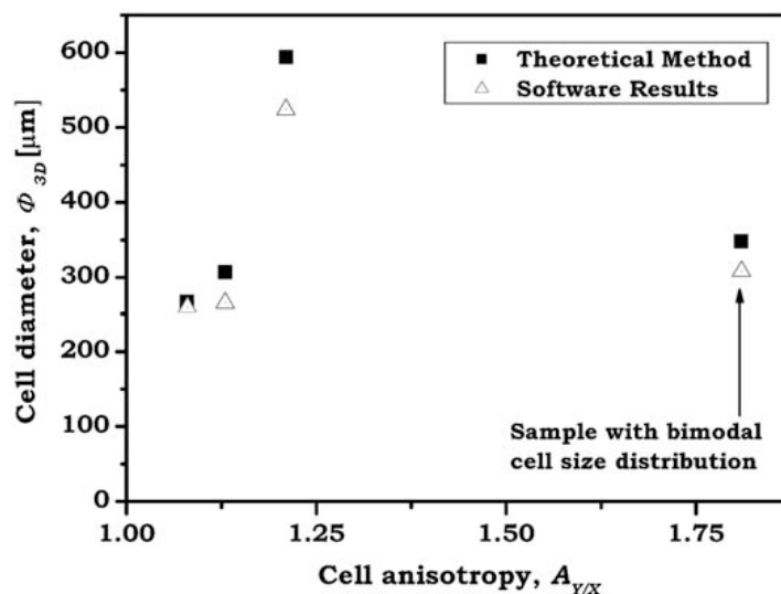
Figure 10. Influence of the cell anisotropy on the agreement between theoretical estimations and experimental results.
