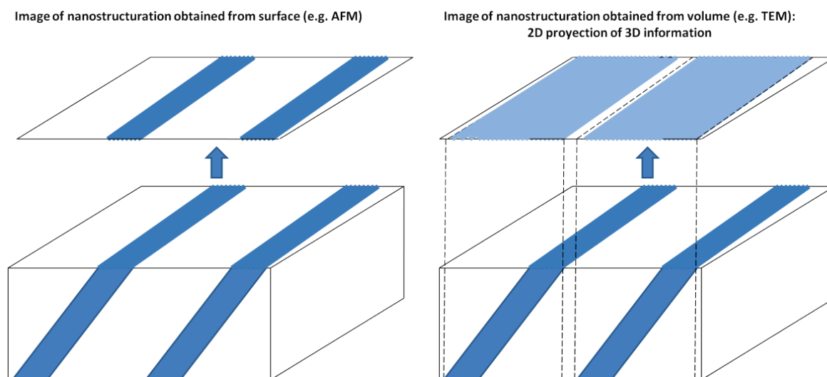
Figure II.7: Difference between the nanostructuring information obtained from a surface (left) and from the entire volume (right) of the sample
