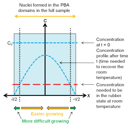
Figure III.4: Schematic model of the solid skin formation on foams presenting heterogeneous nucleation. Sample is extracted of the pressure vessel at time = 0 and foaming starts at time = t . Gas concentration is shown on axis Y, while the sample's width is shown on axis X (center of the sample corresponds to x = 0 ).
