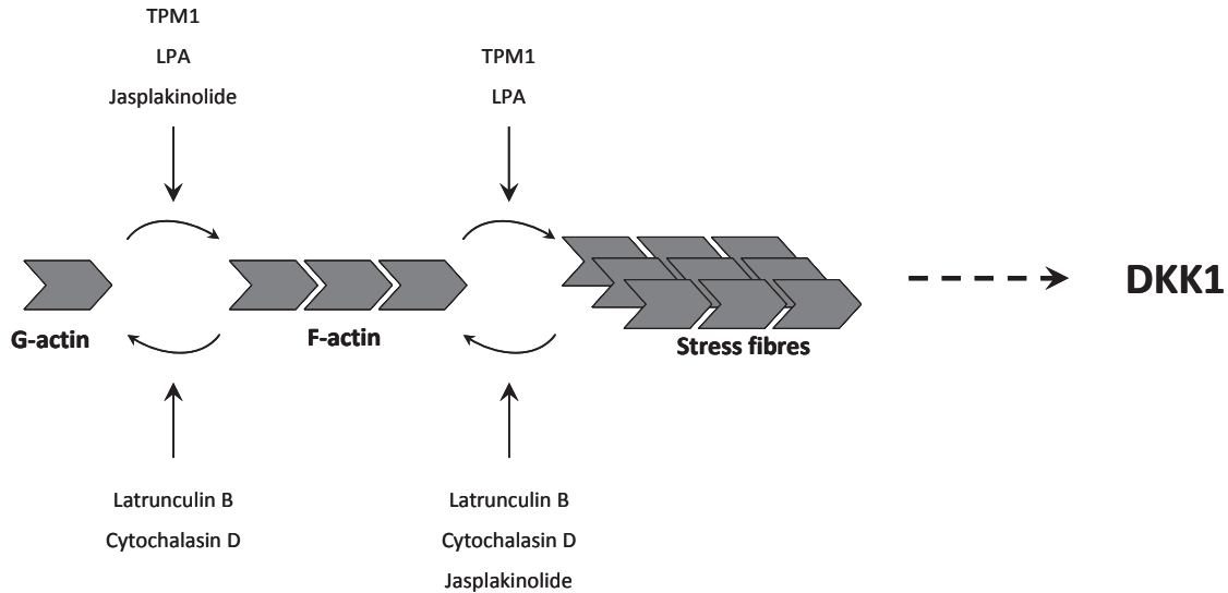
Figure 33. Summary of the major results on the consequences and mechanism of DKK1 downregulation by TNC. (A) TNC reduces DKK1 gene expression in tumor and stromal cells. In tumor cells DKK1 downregulation mediates stimulation of Wnt/ \beta -catenin signalling. In stromal cells the effect of DKK1 downregulation on Wnt/ \beta -catenin signalling needs to be analysed in further detail. (B) Model of DKK1 regulation by the actin polymerisation status of the cell. Disruption of stress fibres and actin depolymerisation (Latrunculin B, Cytochalasin D) decreases DKK1 gene expression, while induction of actin polymerisation and stress fibre formation (LPA, TPM1) increases DKK1 gene expression. Jasplakinolide-mediated actin polymerisation, but stress fibre disruption decreases DKK1 gene expression.
