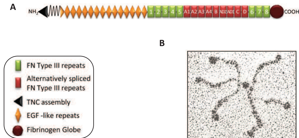
Figure 3. Domain structure of TNC. (A) Organization of TNC into different protein domains. (B) The appearance of purified TNC protein as a hexamer upon electron microscopy (Orend et al. , 2013; Van Obberghen-Schilling et al. , 2011).
