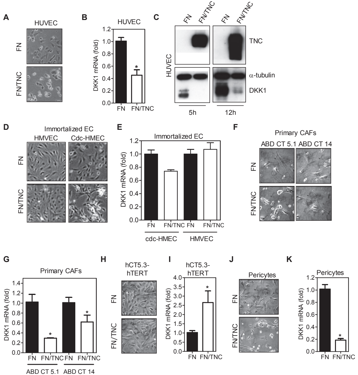
Figure 15. TNC downregulates DKK1 in primary endothelial cells (HUVEC), pericytes and CRC-derived CAF.
