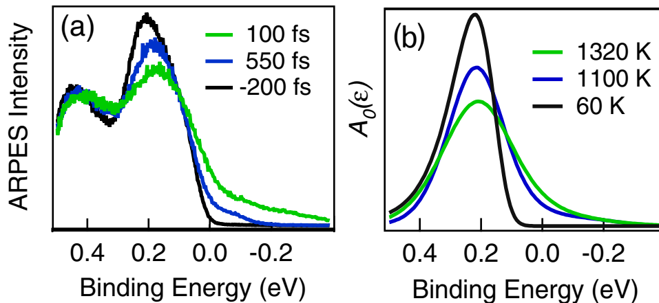
Fig. 2.6: a) 1T-TaS 2 Time-resolved photoemission spectra for a delay of 100 fs, 550 fs and -200 fs. b) Spectral function calculated with DMFT for electrons heated at 1320 K, 1100 K, and 60 K (from [146])
