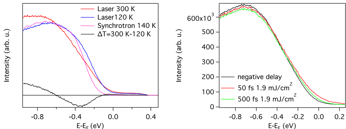
Fig. 5.21: Photoemission spectra near \Gamma for BaCoS 2 using laser and synchrotron. Spectra for different delay times. The laser spectra are similar to the Synchrotron spectra. The photoexcited spectra show in-gap states.
