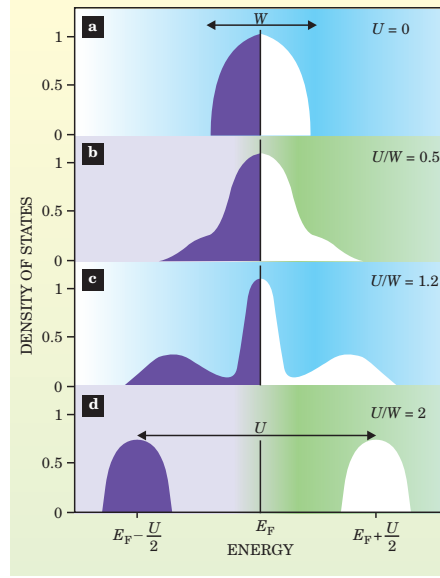
Fig. 1.4: Density of states for different U/W values in the case of the Hubbard model at half filling (from [105])
