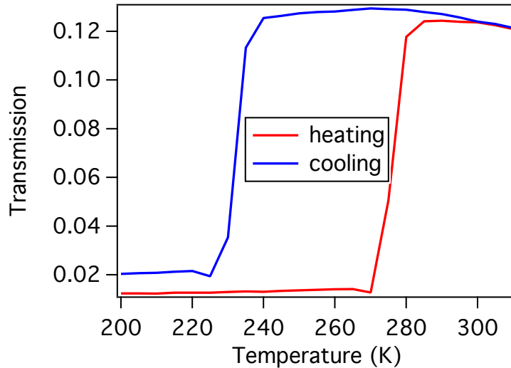
Fig. 5.2: The equilibrium THz transmission in the hysteresis cycle of (V_{1-x}Cr_x)_2O_3 ( x=0.011 ), red being the heating and blue the cooling.
