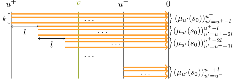
Figure 4.15: Parallel simulation of trajectories estimating (\mu_u(s_0))_{u=u^-}^{u^+} with reuse of trajectories
