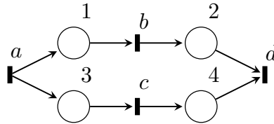
Figure 2.8: A simple Petri net
