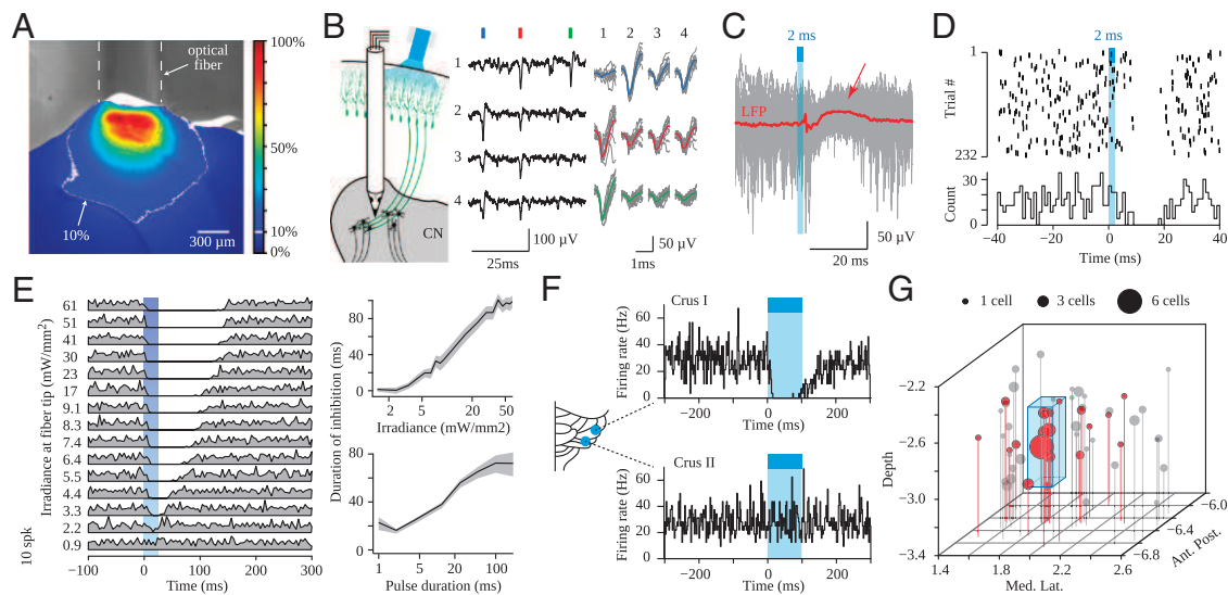
Fig. 3. Effective silencing of cerebellar nuclear cells by photostimulation of Purkinje cells in vivo. (A) Propagation of blue light in the cerebellar cortex (color coded part of the image) for a 600- \mu\text{m} optical fiber placed on the surface of the cerebellum (grayscale part of the image). In the color-coded part, the color of each pixel corresponds to its value expressed as a percentage of the intensity of the brightest pixel. The 10% iseline is delineated in white (i.e., corresponding to \sim 2 \text{ mW/mm}^2 if the brightest pixel immediately under the fiber corresponds to 20 \text{ mW/mm}^2 ). (B) Illustration of tetrode recordings in cerebellar nuclei. (Left) Schematics of the experiment. (Center) Example traces (vertical ticks of different colors signal different spikes; numbers identify the four channels of the tetrode). (Right) Average unfiltered waveforms on the four channels (same color code as for Center), superimposed on 10 successive events (gray traces). (C) Example of a recording obtained on one channel in the interposed nucleus. The average extracellular potential (LFP, local field potential, red) recorded in CN is superimposed on 30 successive sweeps (gray lines) aligned on the onset of photo-stimulation (2 ms, 60 \text{ mW/mm}^2 ). Note the suppression of extracellular (negative) spikes after the stimulation. The average LFP was calculated from 232 sweeps. The red arrow signals the deflection of LFP. (D) Example of a raster plot (Upper) and corresponding PSTH (Lower; bin, 1 ms), showing a complete suppression of firing following the stimulation (blue bar); the example is the same as in C. (E, Left) Example of PSTHs for one cell tested with different light intensities (pulse duration, 25 ms). (Right) Average duration of full inhibition plotted against the irradiance at the fiber tip (at 25 ms) or pulse duration (at 60 \text{ mW/mm}^2 ) ( n = 74 cells) (SI Methods). The shaded area indicates the SEM. (F) Example cell inhibited in response to the illumination of Crus I (Upper, PSTH), but not Crus II (Lower, PSTH). Bin, 5 ms. Blue bar, light pulse (100 ms, 60 \text{ mW/mm}^2 ). (G) A 3D view of the distribution of CN recording sites where inhibited cells were found (red) or not (gray) during Crus I illumination (100 ms, 19 \text{ mW/mm}^2 ) on the ipsilateral cerebellar Crus I region (AP, -6.1 ; ML, 3.3 ). The 3D rectangle arrow identifies the region where most responsive sites are clustered. See Fig. S3 planar projections.
