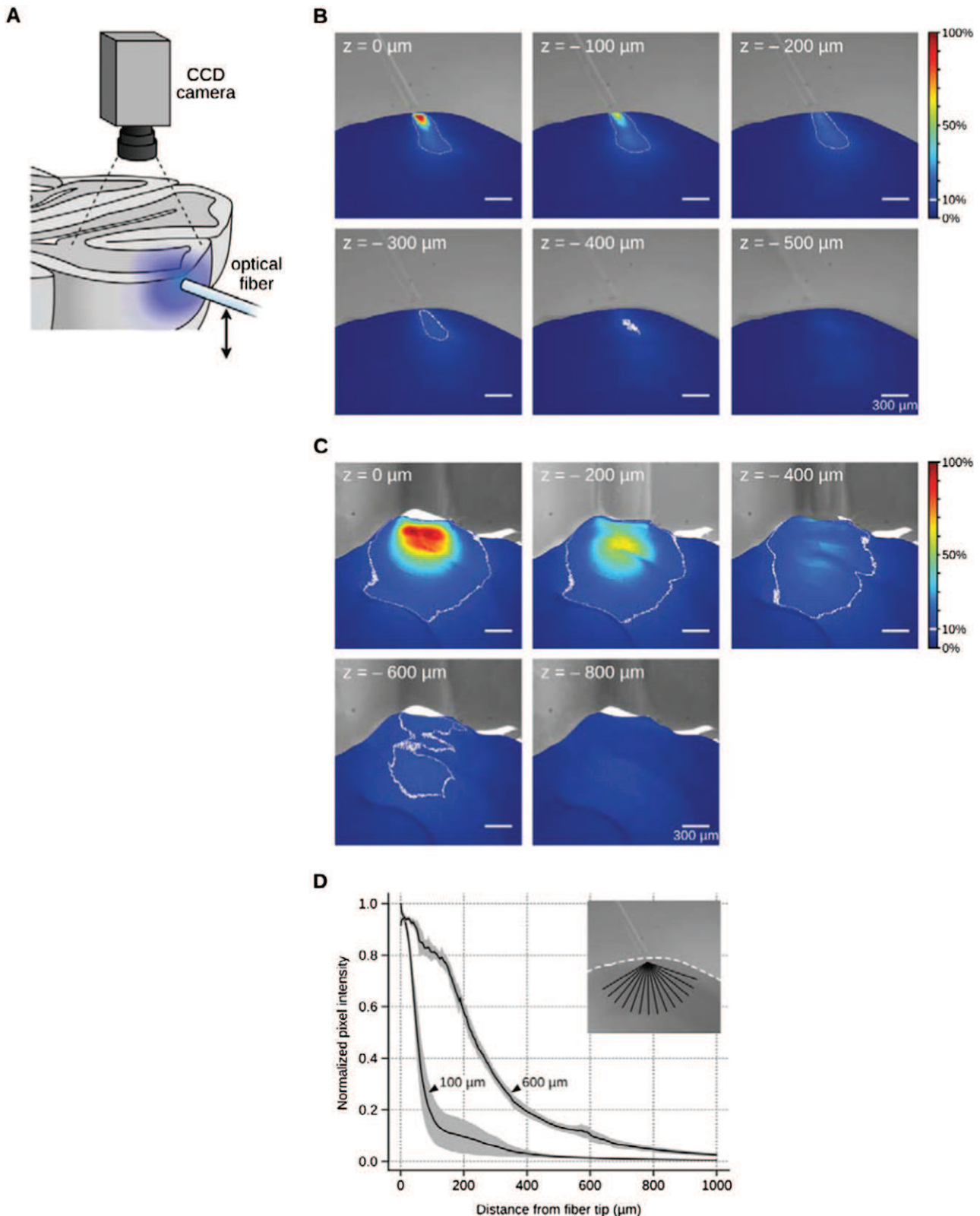
Fig. S5. Light power density mapping using cerebellar hemisections. (A) Schematic of the experimental setup. The cut surface was imaged from the top using a CCD camera whereas the tissue was illuminated from the side through an optical fiber coupled to blue (470 nm) LED. The fiber was translated vertically (two headed arrow) to assess the lateral propagation of light. (B) Series of images taken for different vertical fiber positions using a 100- \mu\text{m} optical fiber with an angle of incidence of \sim 30^\circ and a distance to the pia of around 100 \mu\text{m} . The position of the fiber relative to the cut surface is indicated in white. Pictures were taken in the dark with a power at the fiber tip of 125 \mu\text{W} . The intensity of each pixel is expressed as a percentage of the intensity of the brightest pixel of the image series and color coded. The 10% isoleine is delineated in white on each image. The color-coded image of the tissue is superimposed on a grayscale picture. Legend continued on following page
