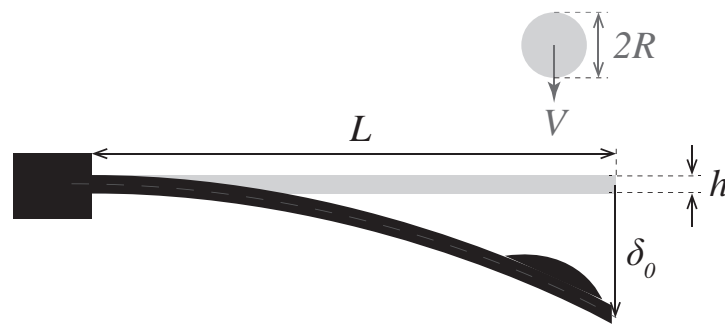
Figure V.6 – Sketch of lamella sensor. A thin glass lamella of length L = 50 mm, thickness h = 160 \mu\text{m} and transverse width b = 24 mm is clamped at one end and free to vibrate at the other one. A drop of radius R and speed V impacts a few millimeters from the tip of the plate. In grey, the system before impact; in black, the system at the maximum deflection \delta_0 . We observe that the drop is sticking to the free end of the plate.
