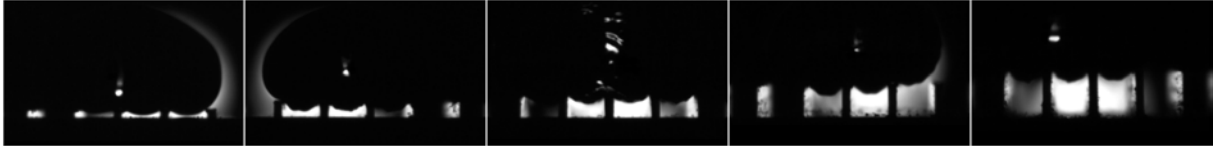
Figure I.25 – Side zoom view of a Leidenfrost puddle drop sitting on crenels of fixed width W = 1 \text{ mm} and wall thickness \lambda = 0.2 \text{ mm} . Depth H from left to right is 200 \mu\text{m} , 400 \mu\text{m} , 600 \mu\text{m} , 800 \mu\text{m} and 1200 \mu\text{m} . On the left image, where H = 200 \mu\text{m} < h , \epsilon is smaller due to the vapor cushion overpressure.
