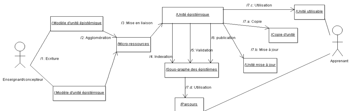
Figure 35 : diagramme de collaboration
