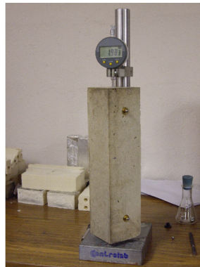
FIGURE B.1: Essais de dessiccation
