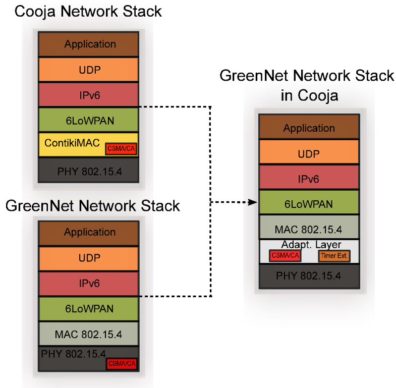
Figure 4.6: GREENNET Network Stack in Cooja
