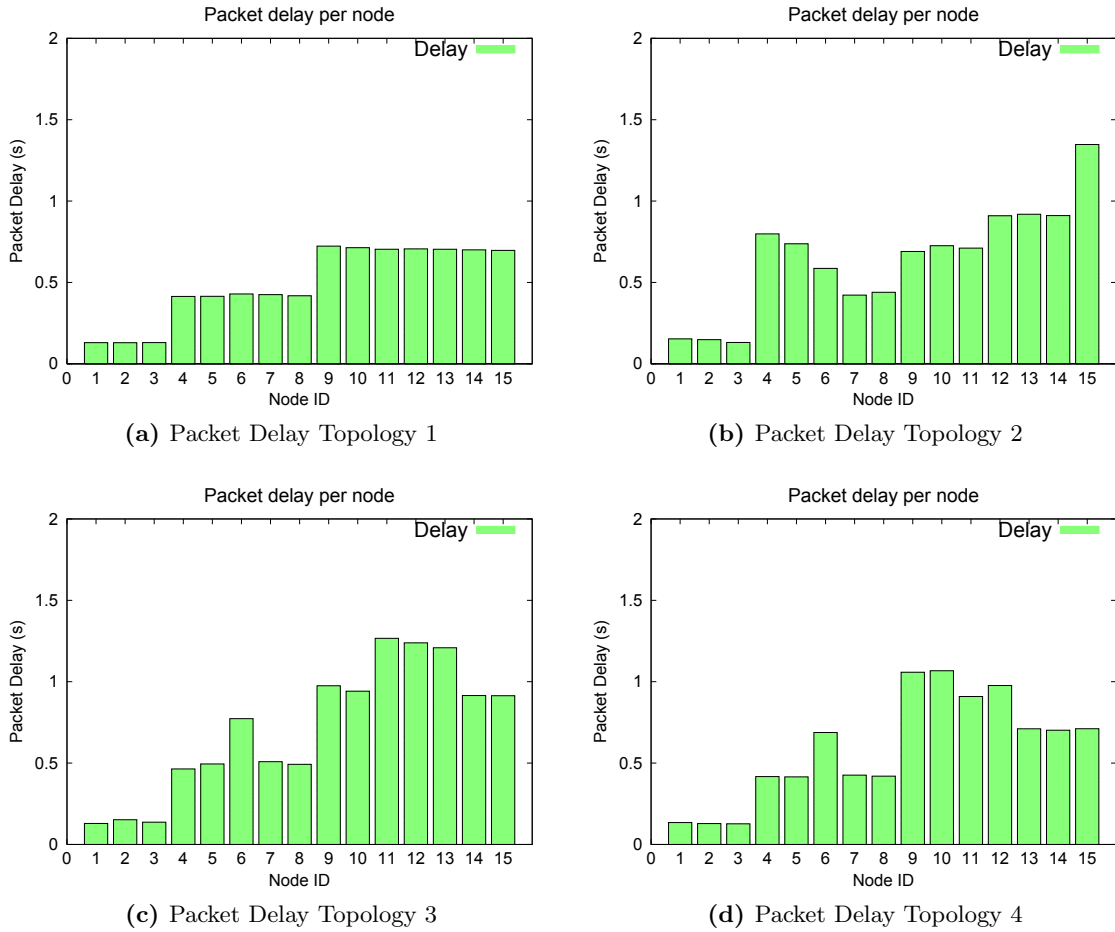
Figure 5.5: Packet delay in different topologies
