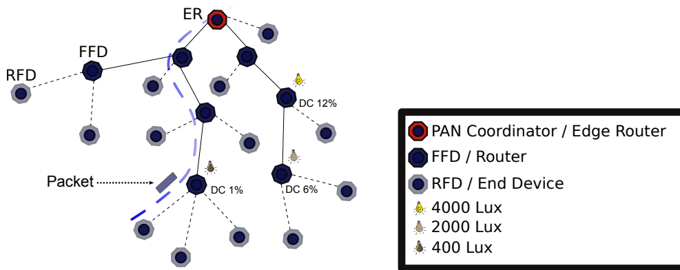
Figure 2.1: GREENNET network
