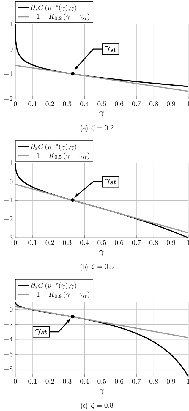
FIGURE 3.5 – Graphical representation of \partial_x G(p^{+*}(\gamma), \gamma) and its tangent function -1 - K(\gamma - \gamma_{st}) around the static oscillation threshold for \zeta = 0.2, 0.5 and 0.8 .
