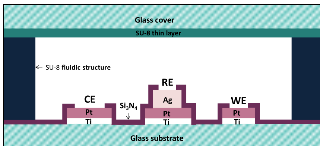
Figure 4.14. Schematic cross section view of the fabricated device.
