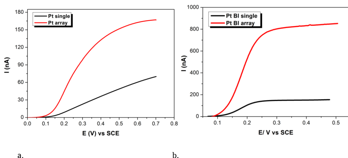
Figure 3.12. Linear sweep voltammograms obtained for (a) Pt and (b) Pt-BI single microelectrodes (black lines) and microelectrode arrays (red lines) in 10 mM of \text{Fe}(\text{CN})_6^{4-} in KCl solution. Scan rate: 4 \text{ mV.s}^{-1} .
