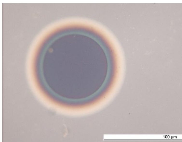
Figure 3.13. \text{IrO}_x film deposited on Pt single microelectrode of 50 \mu\text{m} diameter.
