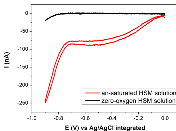
Figure 3.24. Cyclic voltammograms recorded in saturated and zero-oxygen HSM solutions with a Pt-Black UME array. Scan rate: 50 \text{ mV.s}^{-1} .
