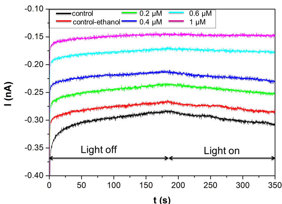
Figure 5.4. Algal response to various concentrations of Diuron herbicide measured with a Pt-BI working ultramicroelectrode array.
