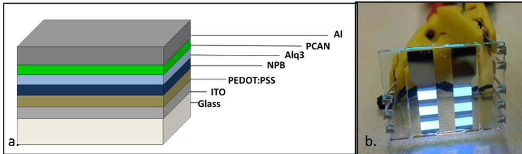
Figure 5.16. (a) OLED composition. (b) Fabricated OLED.
