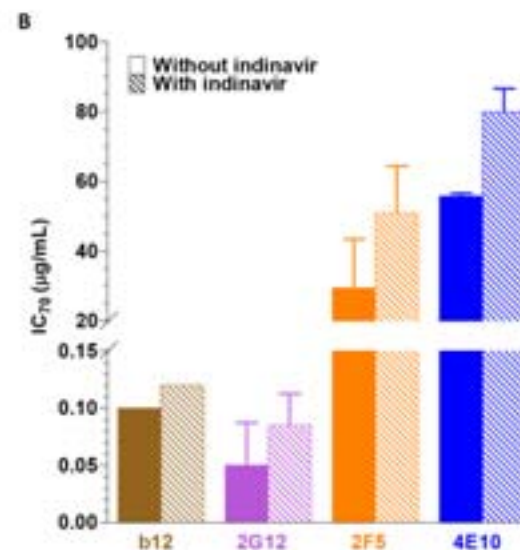
Figure 2: Nabs inhibit HIV-1 trans - and cis -transfer from MDMs to PBLs. Inhibition of (A, B) HIV-1 InE and (C) HIV-1 SF162 transfer by various HIV-1-specific antibodies. Values correspond to (A, C) the percentage of infection in the presence of Abs compared to control without Abs. Dashed line represent IC 70 (Mean ± SD are represented), (B) the IC 70 of NAbs in absence (filled bars) or presence (striated bars) of indinavir (Mean ± SEM are represented).
