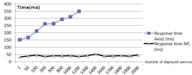
Figure 6.12: Response time evolution- Axis 2 Vs MC (T5 VM template).
