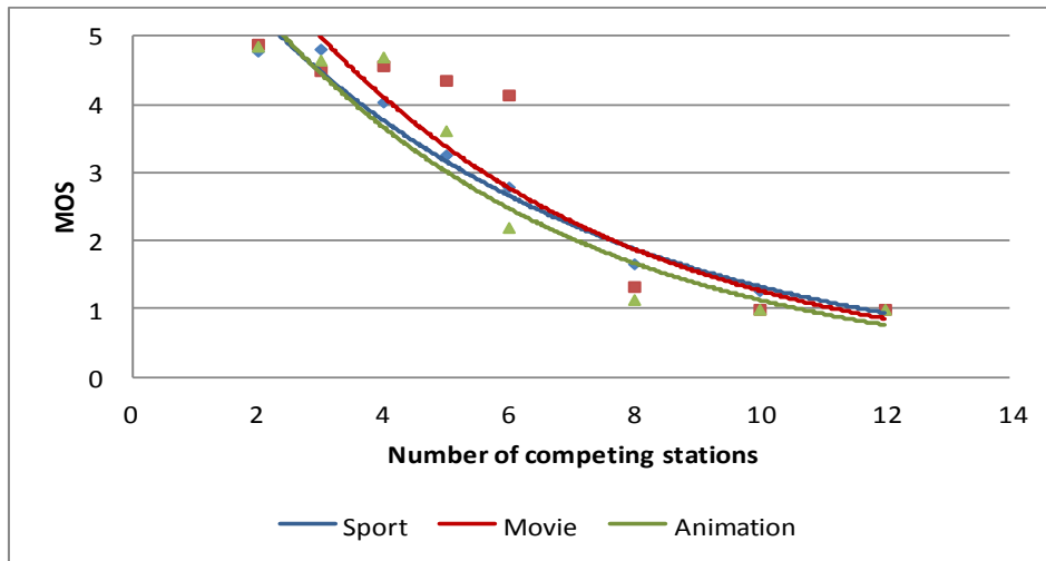
Figure 37: Impact of number of competing stations on video QoE in saturation condition
