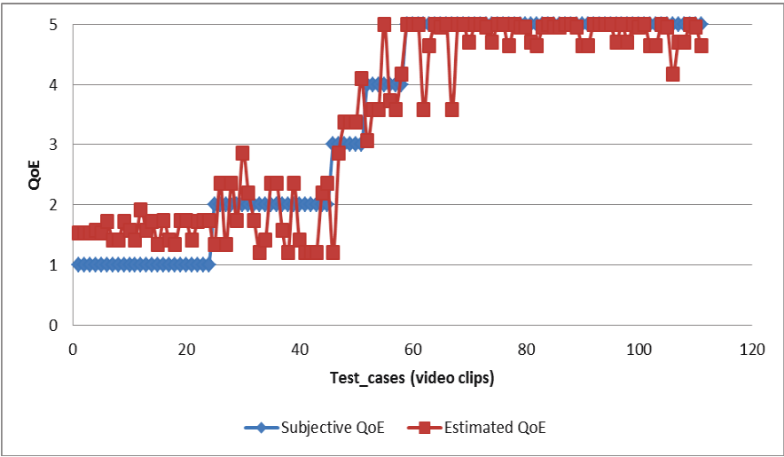
Figure 43: Comparison between subjective and estimated QoE
