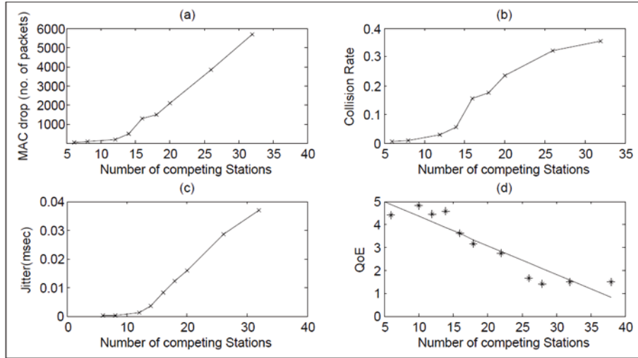
Figure 32: QoS and QoE versus number of competing stations
