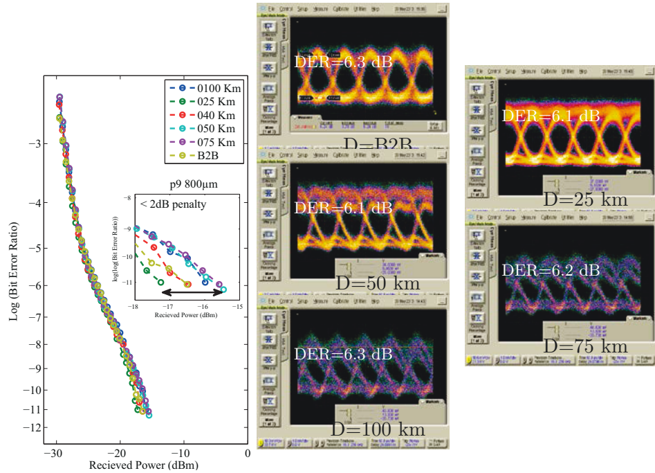
FIGURE 3.38: A standard 10Gbps transmission using a \lambda/4 -phase shifted DFB with p-doped QDash as active material showing transmission up to 100 km with 6 dB extinction ratio.
