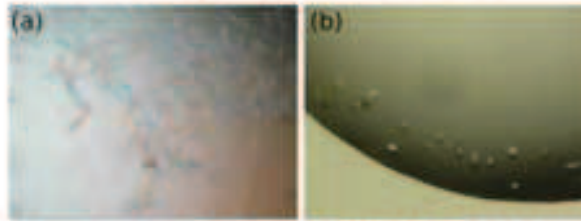
Fig. 5. Crystals of in the same condition with 0.025 mg/ml trypsin added to the protein complex sample.
