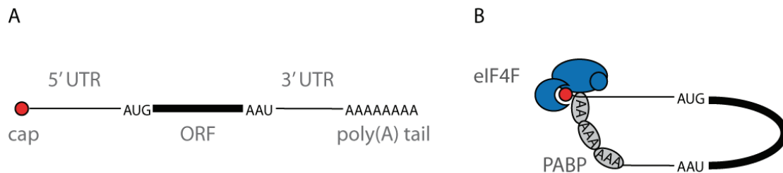
Figure 4 Messenger RNA.
