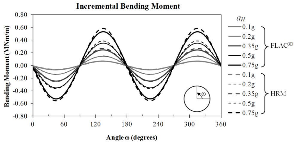
Figure 9-2. Comparison of the incremental bending moment for F = 4.72 , ( R = 2.5\text{m} only seismic-induced loads)
