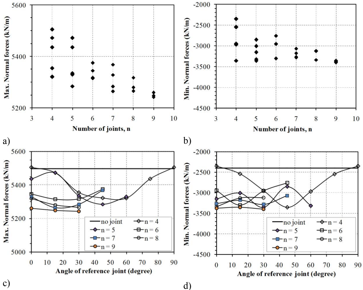
Figure 7-4. The maximum and minimum normal forces vs. joint number and joint orientation, lateral earth pressure factor K_0 equal to 0.5
