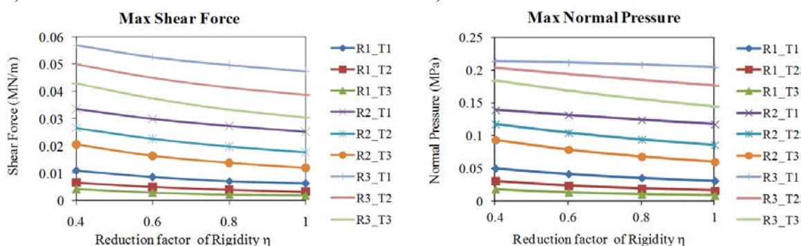
e) Maximum shear force
