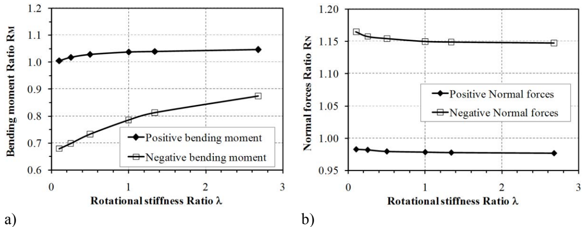
Figure 7-6. The bending moment (a) and normal forces (b) ratio under the influence of the rotational stiffness, joints number equal to 6, lateral earth pressure factor K_0 equal to 0.5
