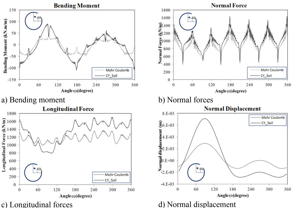
b) Normal forces c) Longitudinal forces d) Normal displacement Figure 5-15. Influence of the constitutive model on the structural lining forces
