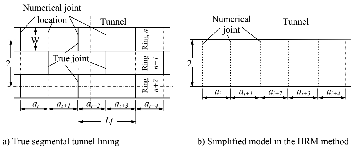
Figure 6-13. Segmental lining scheme
