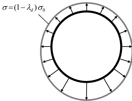
Figure 4-21. Tunnelling simulation with the CCM method (Hejazi et al. [2008])
