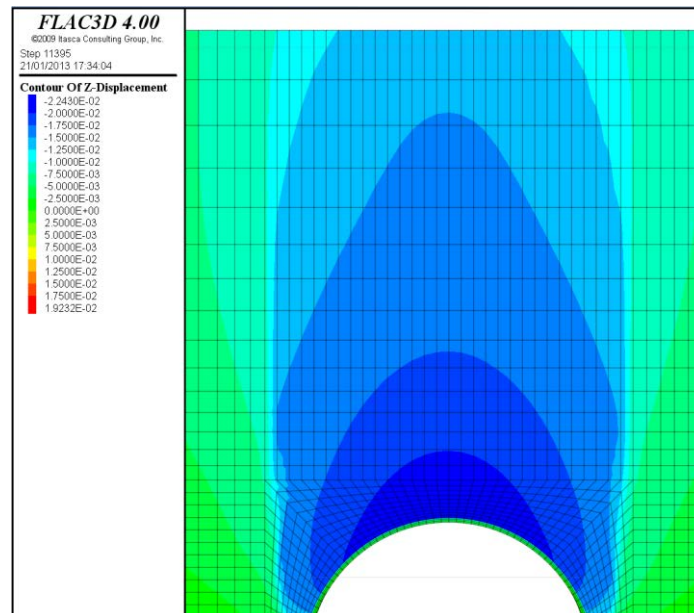
Figure 4-25. Vertical displacement above the tunnel ( \lambda_d value of 0.75)
