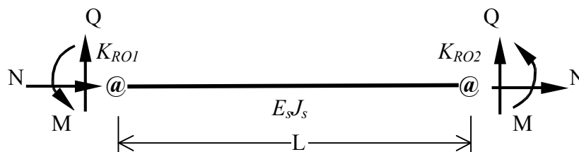
Figure 6-12. Semi-rigid member (Burns et al. [2002])
