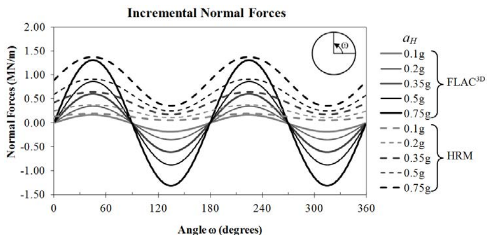
Figure 9-3. Comparison of the incremental normal forces for F = 4.72 , ( R = 2.5\text{m} only seismic-induced loads)
