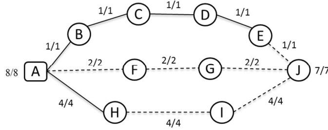
Figure 4:3 A simple disrupted network, where the dashed lines indicate failed arcs
