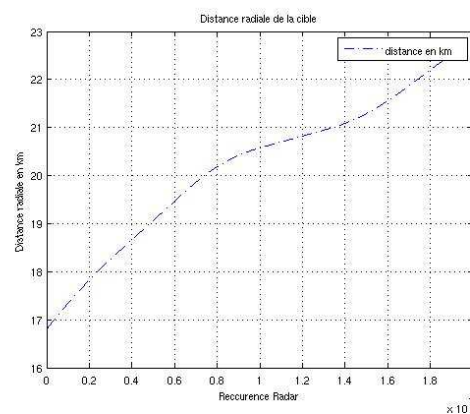
(c) Distance Radar-Cible
