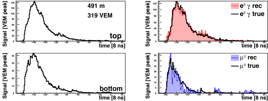
Figure 6.5 Left: simulation of the signal collected in the top and bottom volume of a 10\text{ m}^2 LSD for a 11 EeV shower with 46^\circ zenith angle and 491 m away from the axis. Right: the reconstructed muon and electromagnetic traces compared to the generated ones. The agreement is striking both in shape (timing information of the two components) and amplitude.
