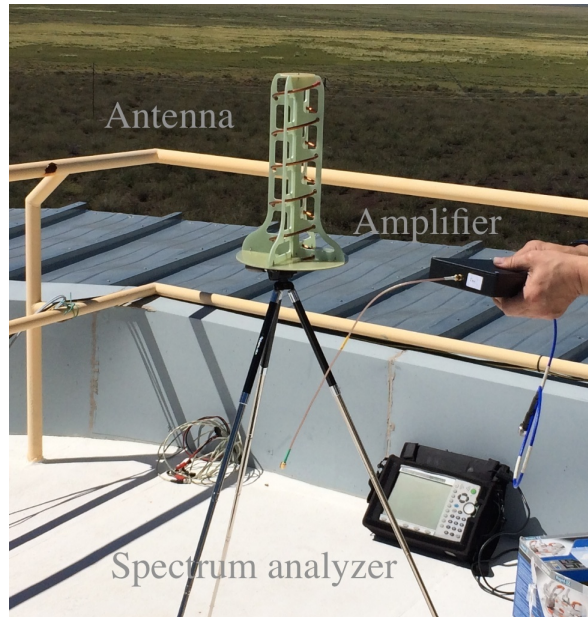
Figure 5.12 Background noise measurements: High Gain Directional Helix antenna, amplifier box (25 dBm) and Anritsu spectrum analyser.
