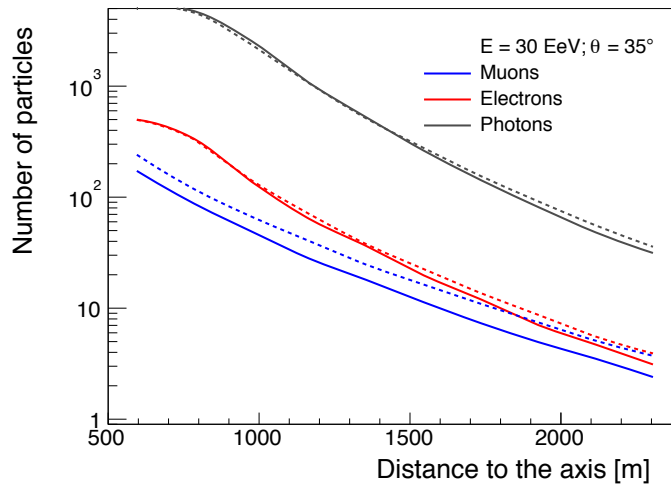
Figure 1.3 Average number of secondary particles hitting a 10 \text{ m}^2 detector according to the distance to the axis for an extensive air shower induced by a proton (solid line) and iron (dashed line) with 30 EeV of energy ( 1 \text{ EeV} = 10^{18} \text{ eV} ) and 35^\circ zenith angle, simulated with QGSJet01.
