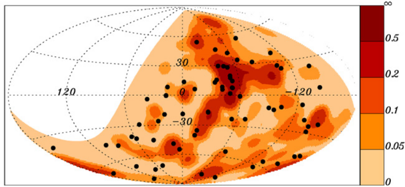
Figure 2.6 Skymap with the arrival directions of 69 Auger events with energy above 55 EeV (filled circles) and with the expected cosmic ray density, smoothed over an angular scale of 5^\circ , derived from a model based on the AGNs in the 58-months Swift-BAT catalog, weighted by their X-ray flux and by the GZK attenuation factor for an energy threshold of 6 \times 10^{19} eV, and by the relative exposure of the observatory. From [124].
