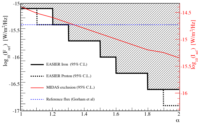
Figure 5.9 Limits set on the MBR flux with EASIER GHz array as a function of the coherence parameter \alpha . The dashed blue line represents the flux measured by Gorham et al. [82]. The solid red line represents the upper limits set with MIDAS detector. The right axis shows I_{ref} = F_{ref} \times 4.62 . From [69].
