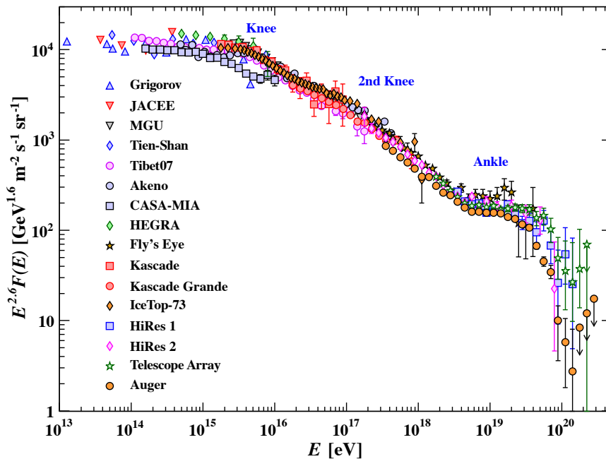
Figure 2.1 Cosmic rays spectrum from 10 13 eV to more than 10 20 eV, as measured by different cosmic ray observatories. The main changes in the evolution of the flux are indicated as the knee , the second knee and the ankle . From [89].
