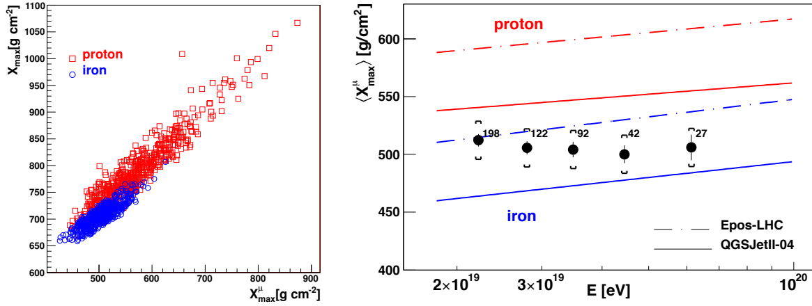
Figure 3.8 Left: X_{\max}^{\mu} versus X_{\max} for simulated proton and iron. Right: the measured X_{\max}^{\mu} presented for different energies compared with different hadronic interaction models. From [144].
