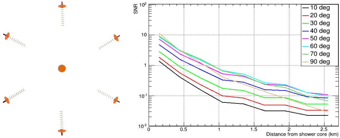
Figure 5.11 Left: configuration of the Giga Duck hexagon, with the exterior antennae pointing to the center at 20° of zenith angle. Right: signal-to-noise ratio (SNR) for the helix antennae for different zenith angles. In the figure is represented 90 - \theta . Simulations by Al Samarai.
