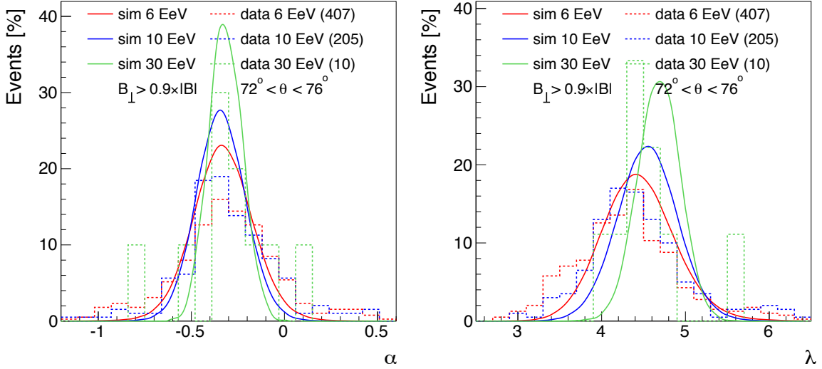
Figure 4.6 Angular distortion parameter \alpha (left) and lateral extension parameter \lambda (right). Normalized histograms for different energies and same zenith angle ( 74^{\circ} ) and B_{\perp} > 0.9|B| . The data are normalized and the lack of large statistics is clear for higher energies, as it is for larger \theta . The number of events is shown between parenthesis. The simulated primaries are protons generated with QGSJet01.
