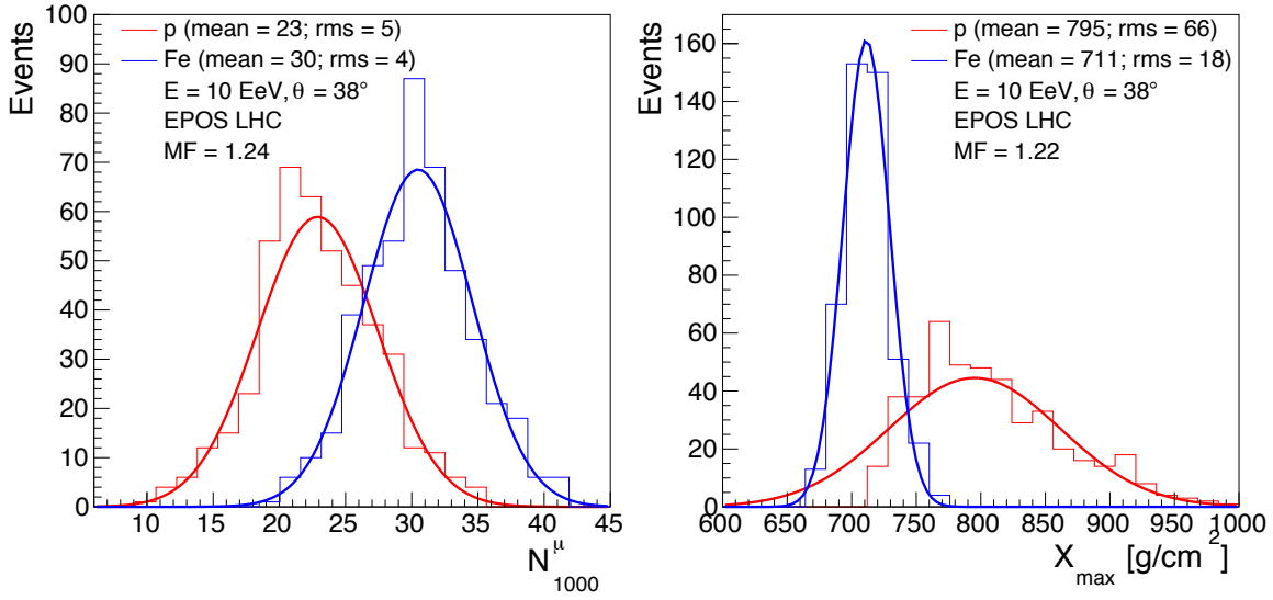
Figure 3.2 Distribution of N_{1000}^{\mu} (left) and X_{\max} (right) for protons and iron nuclei (10 EeV and 38^\circ ). Showers have been simulated with EPOS LHC. The mean and the rms of the distributions are between parenthesis. The merit factor (MF) is indicated (see text for the definition).
