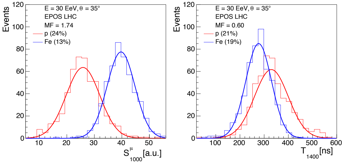
Figure 6.7 Distribution of the observables S_{1000}^{\mu} (left) and T_{1400} (right) for the two different primaries. Showers simulated with EPOS LHC with 30 EeV and 35^\circ zenith angle. The resolutions of the distributions (mean over rms) are between parenthesis. The merit factor (MF) is indicated.
