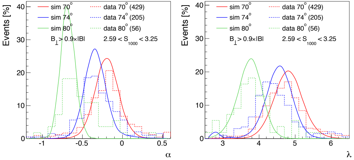
Figure 4.5 Angular distortion parameter \alpha (left) and lateral extension parameter \lambda (right). Histograms for different zenith angles and same energy (10 EeV) and B_\perp > 0.9|B| for protons generated with QGSJet01 and for the Auger data. The sizes of the distributions are normalized to facilitate the comparison, but the decreasing of the available events with higher \theta is clear: the numbers between parenthesis indicate the statistics.
