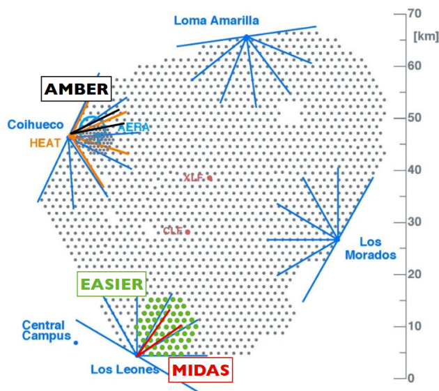
Figure 5.2 Map with the different experiments measuring radio emissions of extensive air showers at Auger.
