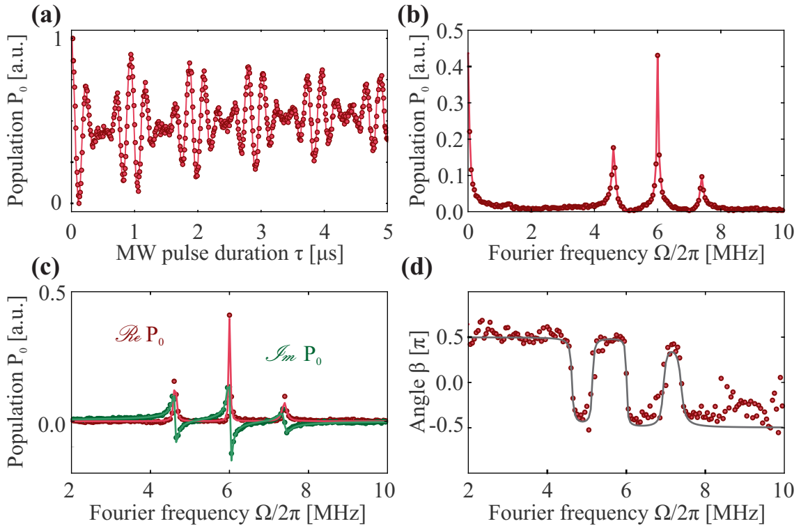
Figure 3.43: Phonon Mollow triplet. (a) Temporal trace of the same Rabi measurement as shown in Figure 3.34. (b) Absolute values of the discrete Fourier transform of (a) The curve is the same as already shown in Figure 3.35. The solid lines in (a) and (b) are guides to the eye. (c) Real (red) and imaginary (green) parts of the Fourier transform of (b) fitted to expression (3.85) (solid lines). (d) Phase of the Mollow triplet. Red points represent data, the grey solid line represents the phase obtained from expression (3.85) with the fitting values obtained from (c).
