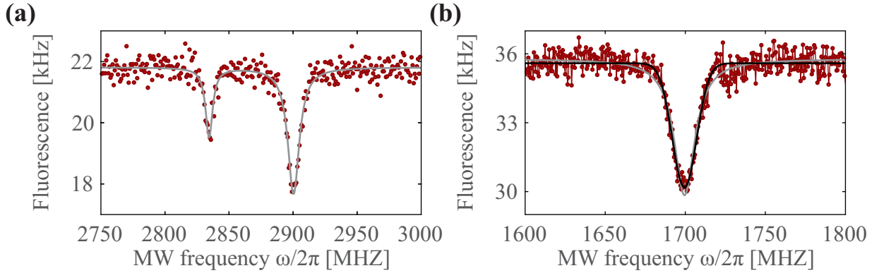
Figure 4.12: ODMR measurements of the NV spin. (a) Far away from the magnetic structure, the spin couples only weakly to the oscillator position and the |+1\rangle and | -1\rangle eigenstates are mainly split due to strain effects in the nanodiamond. The gray line is a fit two a sum of two Lorentzian lineshapes. (b) Closer to the magnetic structure, the magnetic field and magnetic field gradient increase, shifting the |+1\rangle eigenstate close to the ESLAC ( B_{\parallel}^{\text{ext}} \approx 51 mT). ESR spectra, taken over several minutes, are then experiencing additional broadening due to thermal drifts, which slowly shift the spin resonance frequency \omega_0/2\pi in an inhomogeneous manner. The gray line indicates a fit to a Lorentzian lineshape, while the black curve is a fit to a Gaussian lineshape. The difference in fluorescence is due to different optical powers.
