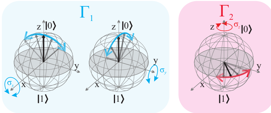
Figure 2.15: The effect of external noise on spin populations ( \Gamma_1 ) and coherences ( \Gamma_2 ).
