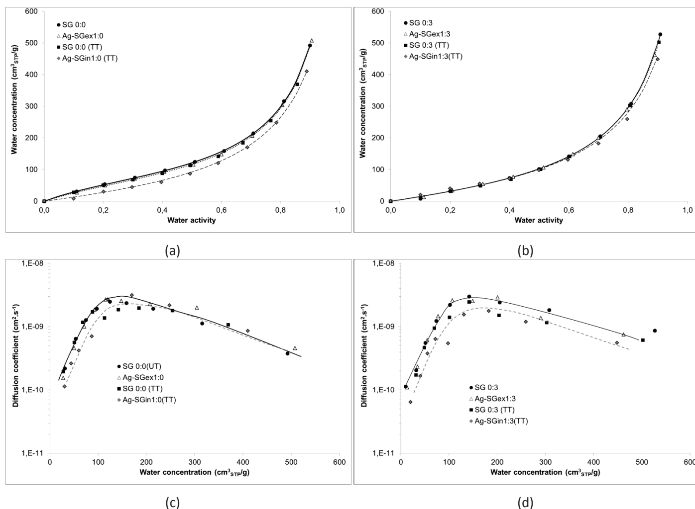
Figure 7: Water sorption properties of the different nanocomposite films using different AgNO 3 /Glucose molar ratio (1:3 and 1:0) and associated neat starch matrix: (a),(b) the water concentration at equilibrium versus the water activity and (c),(d) the diffusion coefficient versus the water concentration at equilibrium
