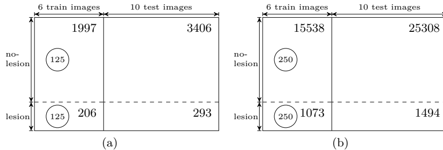
Figure 3.33: Randomized sampling for classifier training from the pool of superpixels. The values represent the amount of superpixels and the circle illustrate the random selection for a training round. The superpixels' pool correspond to case of: (a) Quick-Shift (QS), (b) Global Probability Boundary (gPb).
