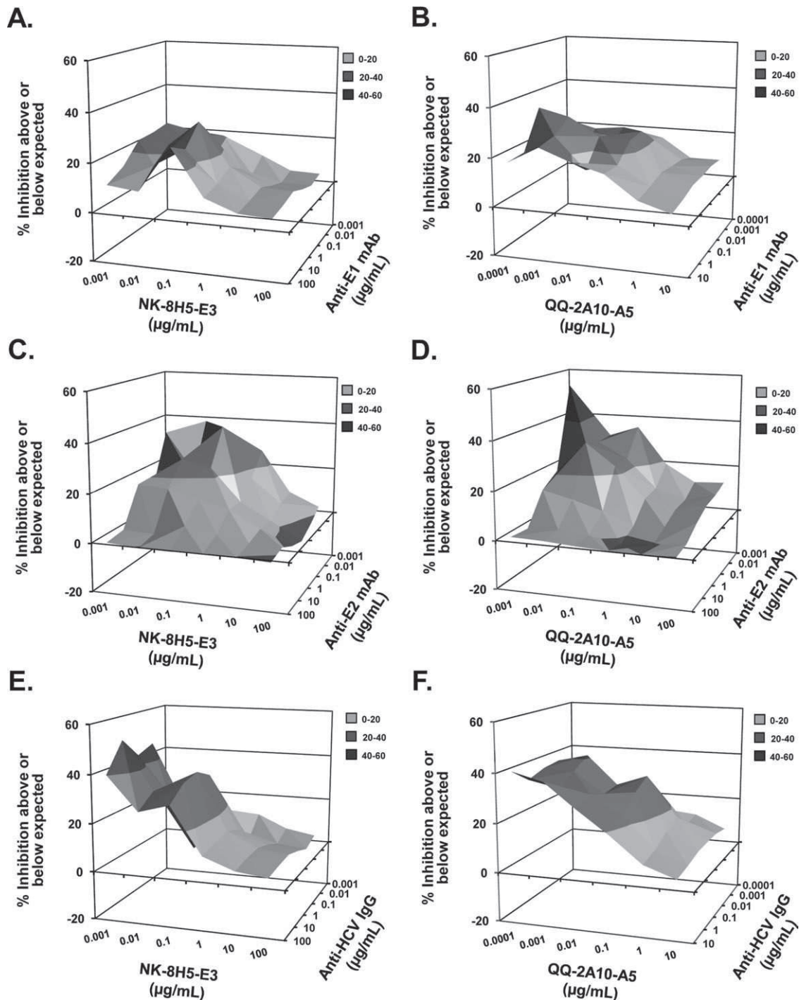
Fig. 6. Synergy between anti-SR-BI and neutralizing antibodies in inhibiting HCV infection. HCVcc (Luc-Jc1) were preincubated with increasing concentrations of (A,B) anti-E1 (IGH520) or (C,D) anti-E2 (AP33) mAbs or (E,F) purified heterologous anti-HCV IgG obtained from an unrelated chronically infected subject or isotype control IgGs for 1 hour at 37°C and added to Huh7.5.1 cells preincubated with increasing concentrations of control or anti-SR-BI mAbs (A,C,E) NK-8H5-E3 or (B,D,F) QQ-2A10-A5 in a checkerboard format. HCVcc infection was analyzed by luciferase reporter gene expression. Effects of antibody combinations on HCVcc infection were evaluated using the method of Prichard and Shipman. 32 Combination studies for each pair of compounds were performed in triplicate. The theoretical additive effect is calculated from the dose-response curves of individual compounds using the equation z = x + y(1 - x) , where x and y represent the inhibition produced by the individual compounds and z represents the effect produced by the combination of compounds. The theoretical additive surface is subtracted from the actual experimental surface, resulting in a horizontal surface that equals the zero plane when the combination is additive. A surface raising more than 20% above the zero plane indicates a synergistic effect of the combination, and a surface dropping lower than 20% below the zero plane indicates antagonism.
