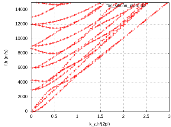
(b) Relation de dispersion.
