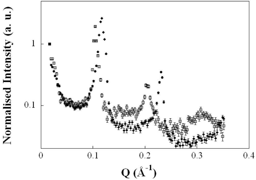
Fig. 8: Diffraction data taken on D16 at ILL to evaluate the d-spacing for two samples with different hydrations levels [56]. Open squares: 100 % rh (pure D 2 O atmosphere); filled diamonds: 75 % rh (D 2 O in saturated NaCl salt solution). The experimental d-spacing are 62.5 Å and 54.9 Å, respectively [56].
