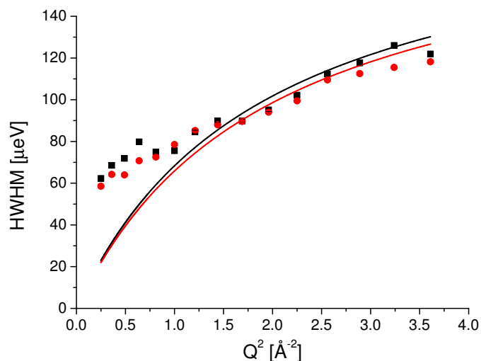
(a) Lorentzian width at a wavelength of 5.1 Å (elastic energy resolution: 90 μeV). Fit curves correspond to equation 3.32 of the jump diffusion model. A clear deviation for low Q -values, corresponding to confinement effects, is visible. The results from the fits are given in table 9.5.
