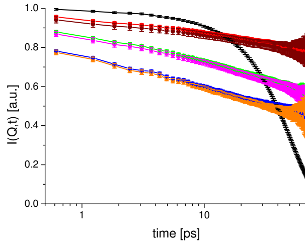
(b) Comparison of I(Q,t) of pure AChE and AChE + HupA ( \lambda = 5.9 \text{ \AA} ). Data for the pure AChE is depicted with squares, AChE + HupA with circles, respectively. Again selected Q -values of 0.5 \text{ \AA}^{-1} (red and brown), 1.0 \text{ \AA}^{-1} (green and pink) and 1.5 \text{ \AA}^{-1} (blue and orange) are shown.
