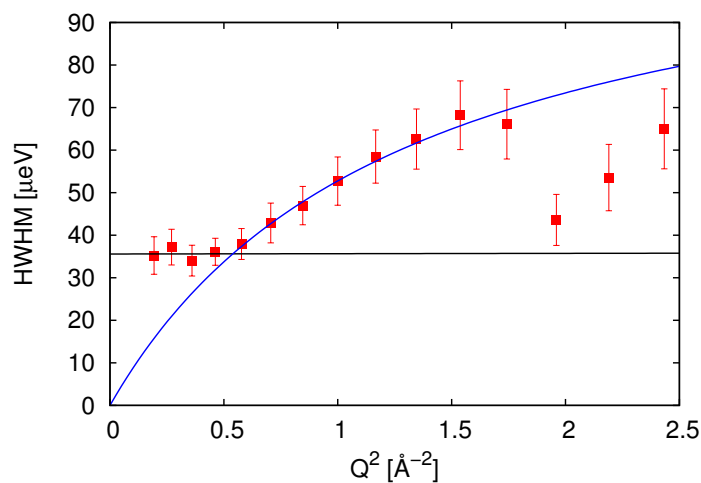
Figure 7.7: Line width of the smaller Lorentzian for the higher hydrated sample at 278 K. A plateau (marked with a black line) indicating a confinement is observed at small Q -values. For high Q -values the data follow a behaviour according to equation 3.32 of the random jump diffusion model (blue curve). Data are fitted up to Q^2 -values of 1.5 \text{ \AA}^{-2} to exclude the influence of the coherent scattering arising from the chain ordering in the gel phase around 2 \text{ \AA}^{-2} .
