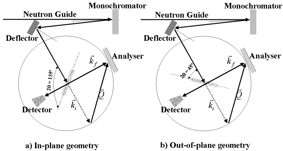
Fig. 1: By rotating the sample with respect to the incoming beam, the momentum transfer is predominantly oriented parallel ( 135^\circ , panel a) and perpendicular to the membrane surface ( 45^\circ , panel b)
