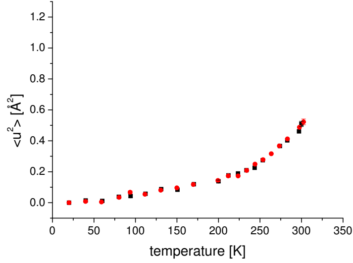
(a) IN6, 90 \mu\text{eV} , t_{\text{max}} \approx 10 ps.
