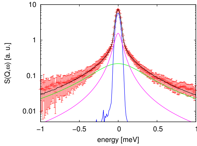
(b) Q = 1.48 \text{ \AA}^{-1} .
