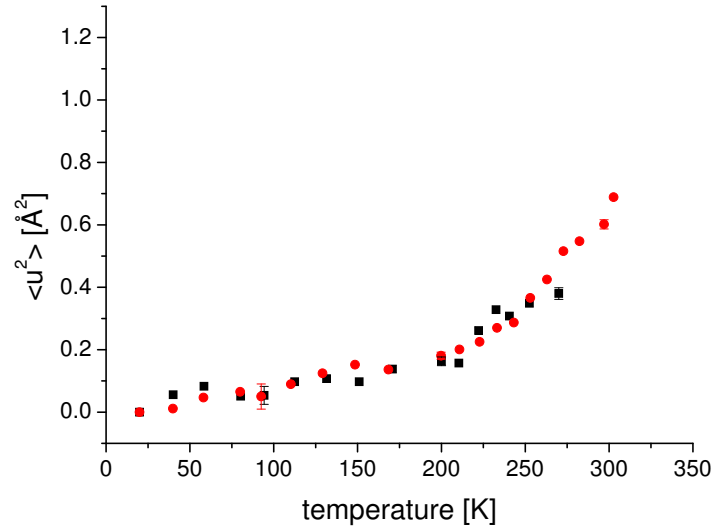
(b) IN6, 50 \mu\text{eV} , t_{\text{max}} \approx 20 ps. Due to limited beamtime the native AChE sample could only be measured up to a temperature of 270 K.
