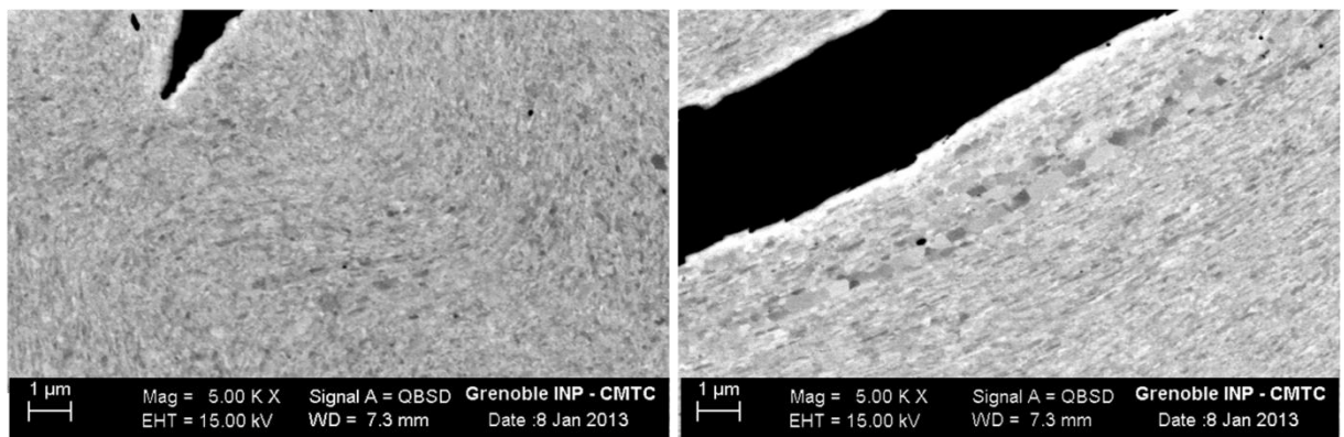
Figure III.15: SEM images of a 12h@600°C annealed powder P9073
