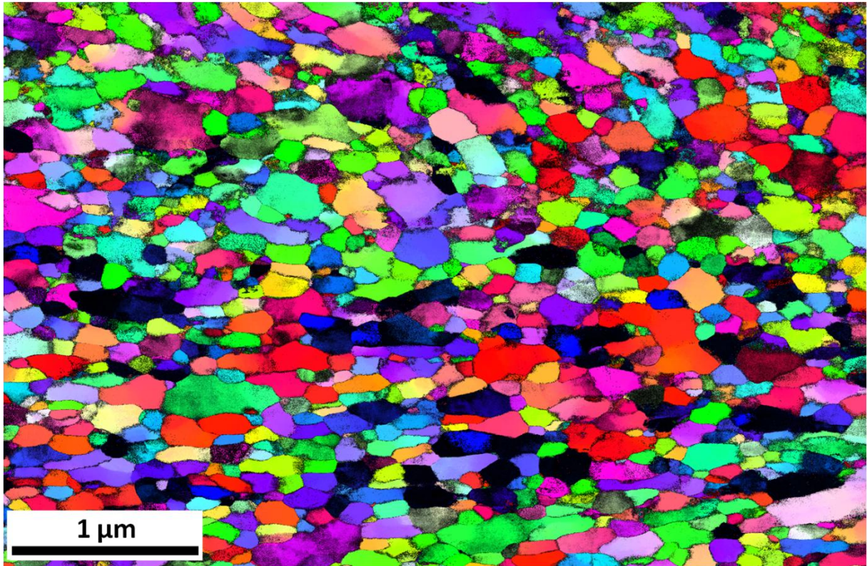
Figure III.27: Microstructure of the P9073 powder after a 5min@800°C annealing
