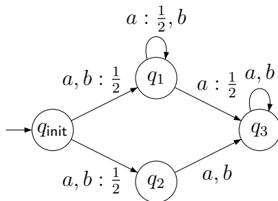
Figure 4.2: The MDP described in Example 4.2 where for the target set T = \{q_1, q_3\} , we have q_{\text{init}} \in \langle\langle 1 \rangle\rangle_{\text{sure}}^{\text{event}}(\text{sum}_T) but q_{\text{init}} \notin \langle\langle 1 \rangle\rangle_{\text{sure}}^{\text{event}}(q_2) .
