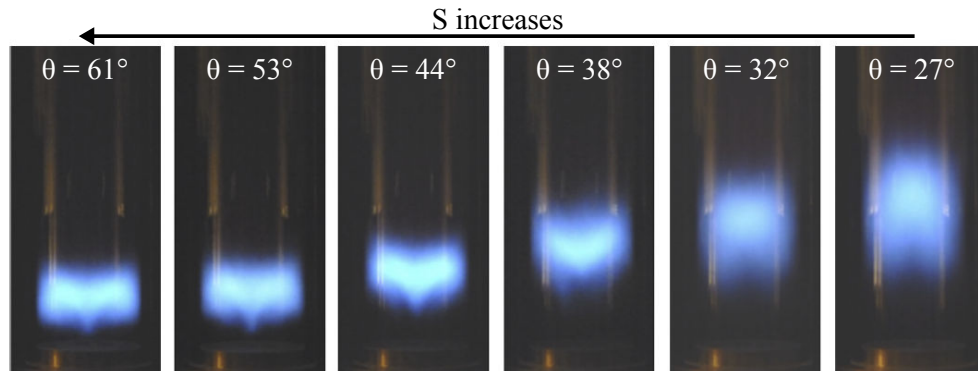
Figure 19: Images of premixed \text{CH}_4/\text{air} flames in an atmospheric laboratory scale burner operated at an equivalence ratio \phi = 0.70 and a bulk flow injection velocity U = 11.0 \text{ m} \cdot \text{s}^{-1} for different swirler blade angles. Adapted from Durox et al. (2013) .
