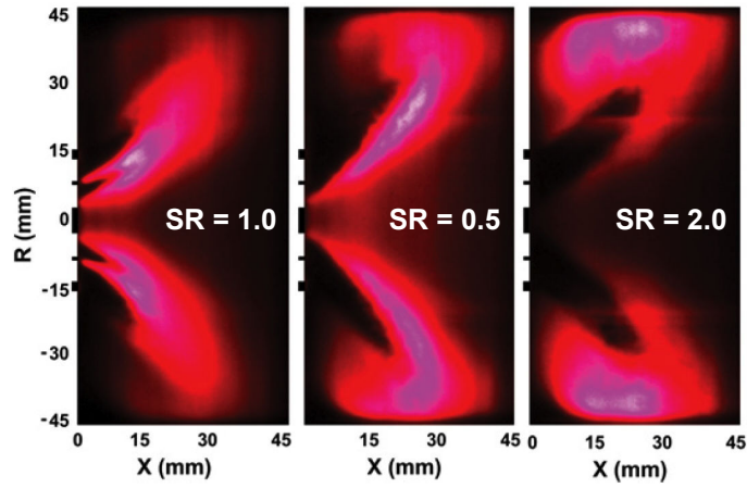
Figure 18: Time-averaged OH-PLIF distribution of atmospheric \text{CH}_4/\text{air} flames featuring different stratification ratios SR defined by the ratio of the inner stream equivalence ratio to the outer stream equivalence ratio. The global equivalence ratio and the bulk flow velocity are fixed to \phi = 0.60 and U = 5 \text{ m} \cdot \text{s}^{-1} . Adapted from Kim and Hochgreb (2012) .
