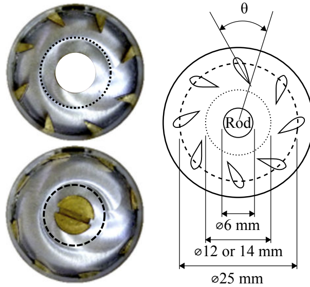
Figure 4.2: Left: top views of the adjustable swirler for a blade angle \theta = 23^\circ (top) and \theta = 61^\circ (bottom) (Durox et al. (2013)). The black dotted and dashed circles represent the 14 mm (configuration A) and 12 mm (configuration B) injection tube diameters respectively. The central hole is crossed by the rod in configuration A and obstructed by a screw in configuration B. Right: Schematic with the main dimensions of the swirler.
