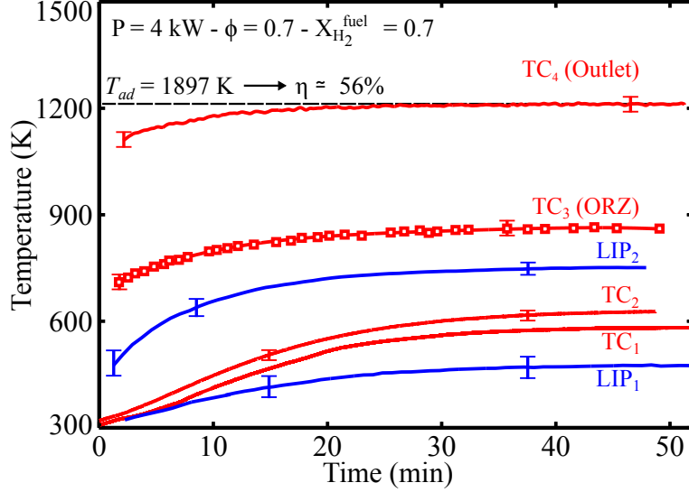
Figure 3.11: Temporal evolution of temperatures reached at the locations indicated in Fig. 3.10 from ignition ( t = 0 ) to steady-state ( t \simeq 45 min) for a \text{CH}_4/\text{H}_2/\text{air} flame at P = 4 kW, X_{\text{H}_2}^{\text{fuel}} = 0.70 , and \phi = 0.7 .
