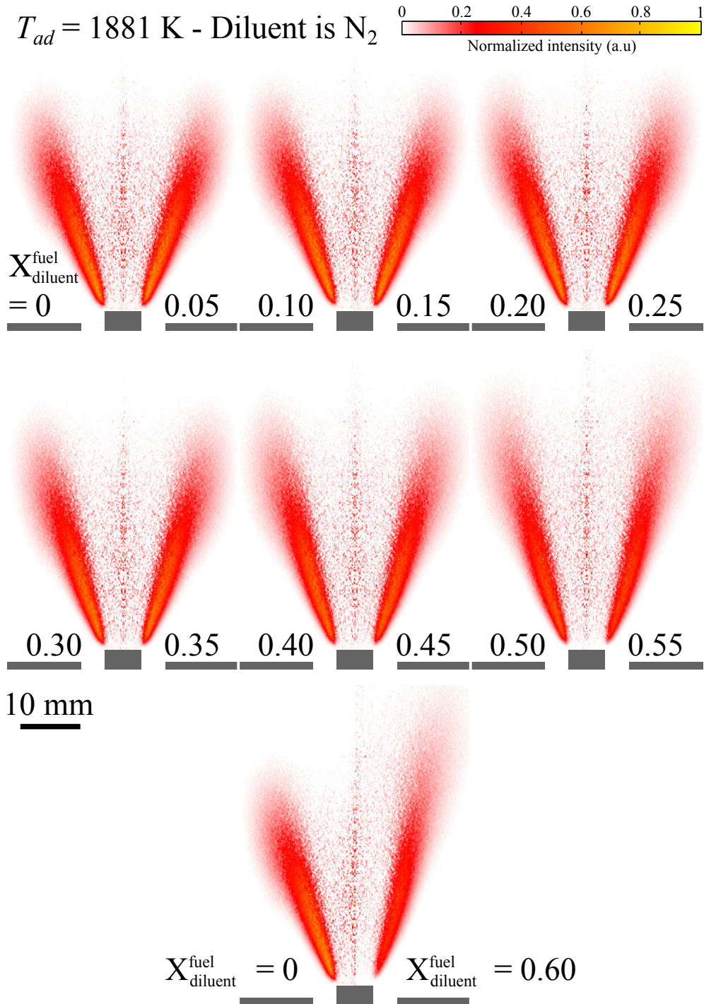
Figure 7.5: Abel transformed \text{OH}^* chemiluminescence images of swirled flames when the molar fraction of \text{N}_2 in the fuel blend is increased (air not included) from X_{\text{diluent}}^{\text{fuel}} = 0 to X_{\text{diluent}}^{\text{fuel}} = 0.60 for a fixed adiabatic flame temperature T_{ad} = 1881 \text{ K} , thermal power P = 4 \text{ kW} , and hydrogen enrichment X_{\text{H}_2}^{\text{fuel}} = 0.60 .
