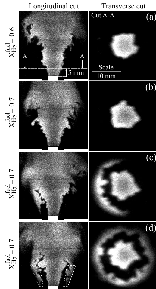
Figure 5.4: Axial (left) and transverse (right) OH-PLIF snapshots for X_{H_2}^{fuel} = 0.60 (a) and X_{H_2}^{fuel} = 0.70 ((b) (c) (d)). The dashed line in (a) indicates the transverse plane used for measurements 5 mm above the central rod tip. Axial and transverse measurements are not synchronized in these images.
