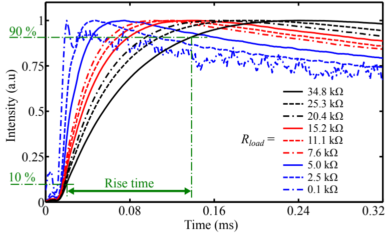
Figure 2.44: Normalized phosphorescent signals obtained using different load resistors for Mg_{3.5}FGeO_5:Mn at T = 290 K. Effects of the load resistor connected to the detector on its rise time is emphasized.
