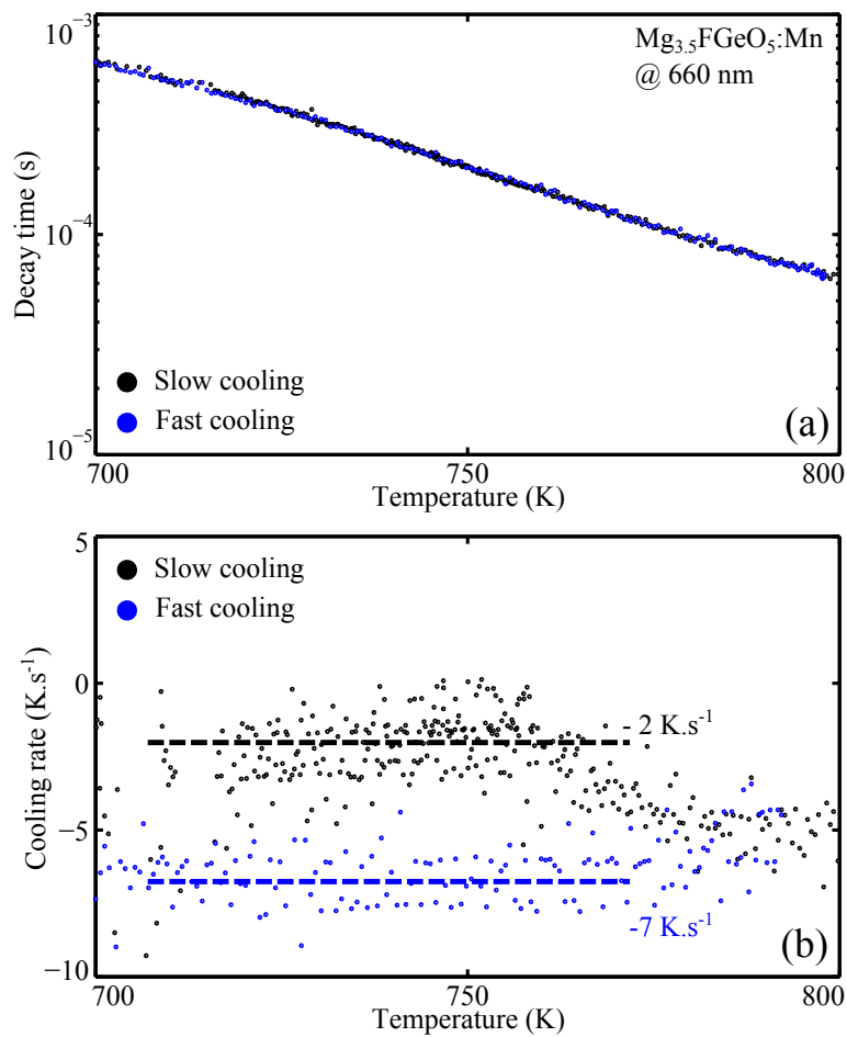
Figure 2.50: (a) Calibration curves for Mg_{3.5}FGeO_5:Mn between 700 K and 800 K using a "slow" (black) and a "fast" (blue) cooling rate of the painted thermocouple. (b) Cooling rate as a function of the temperature for both experiments used to build the calibration curves visible in (a).
