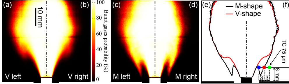
Figure 5.12: Conditional mean of 1080 binarized longitudinal OH-PLIF images giving the probability of presence of hot burnt gases for the flames featuring a V shape at the left (a), a V shape at the right (b), an M shape at the left (c), and an M shape at the right (d) for X_{H_2}^{fuel} = 0.70 . (e)-(f) Contour of the zones featuring a non zero probability of hot burnt gases for the mean V (red) and M shape (black) flames. Dots show the position of the 75 \mu\text{m} type R thermocouple in the OSL (blue), near the GMLI (red), and in the ORZ (green).
