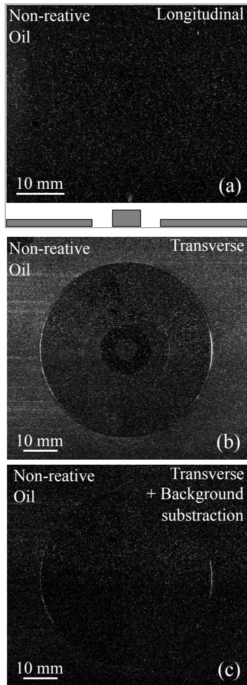
Figure 2.27: Examples of Mie scattering images obtained under non-reactive conditions and using oil as a seeding agent in a longitudinal (a) or a transverse plane (b) and (c). A background subtraction is applied on (c). See the electronic version of this document for a better image definition.
