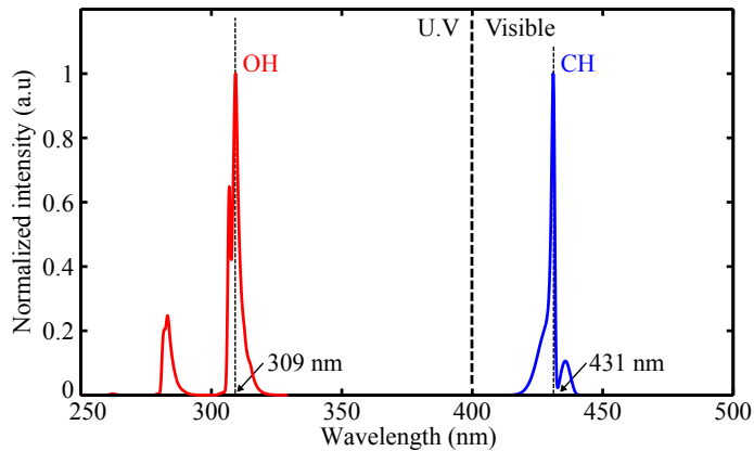
Figure 2.7: Simulated emission spectra of \text{OH}^* and \text{CH}^* radicals at P = 101325 Pa and T = 1850 K using LIFBASE (Luque and Crosley (1999)). Spectra are convoluted using a 1 nm coarse slit function.
