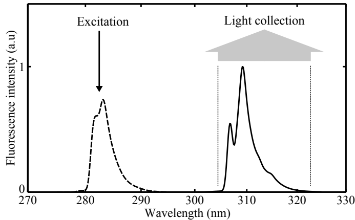
Figure 2.12: Normalized absorption [280 nm - 290 nm] and emission [300 nm - 320 nm] spectra of the OH radical convoluted with a 1 nm coarse slit function using LIFBASE (Luque and Crosley (1999)).
