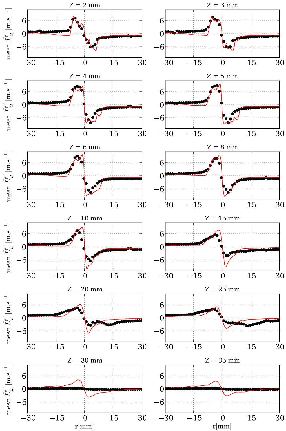
Figure 3.8: 1-D radial mean profiles of the orthonormal velocity component U_y at different heights z above the bluff-body surface in the longitudinal plane Y = 0 mm. Red lines and black symbols respectively correspond to LES calculations and PIV measurements.
