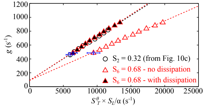
Figure 4.18: Velocity gradient g corresponding to V to M bifurcations as a function of S_T^\theta S_L / \alpha for the aerodynamically stabilized flames ( Le = 0.97 , injector set in configuration B , S_6 = 0.68 ) with (black body triangles) and without (hollow body triangles) accounting for dissipation effects in the flame tube. Values for rod stabilized flames ( Le = 0.97 , injector set in configuration A , S_2 = 0.32 ) are represented by black circles. Dashed lines show linear regressions of the data. The blue error bars give an indication of uncertainties.
