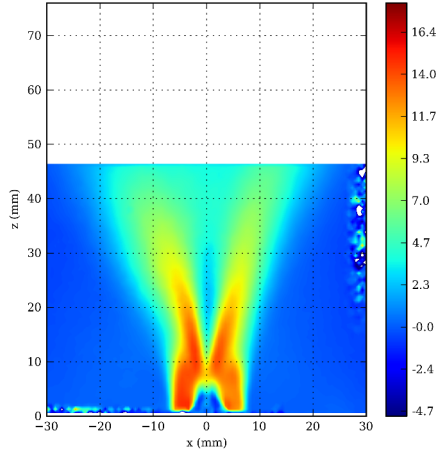
(a) PIV - U_z [m.s -1 ] - Plane Y = 0 mm
