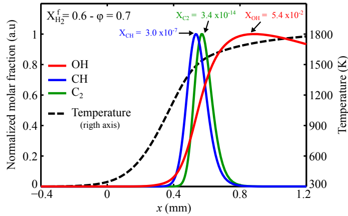
Figure 2.6: Normalized molar fractions of OH, CH, and C_2 as a function of the distance to a one-dimensional laminar flame front of a CH_4/H_2 /air flame ( X_{H_2}^{fuel} = 0.60 and \phi = 0.70 ). right-axis: Evolution of the gas temperature. The REGATH solver (Candel et al. (2011)) was used with the detailed chemistry mechanism from Lindstedt (1998).
