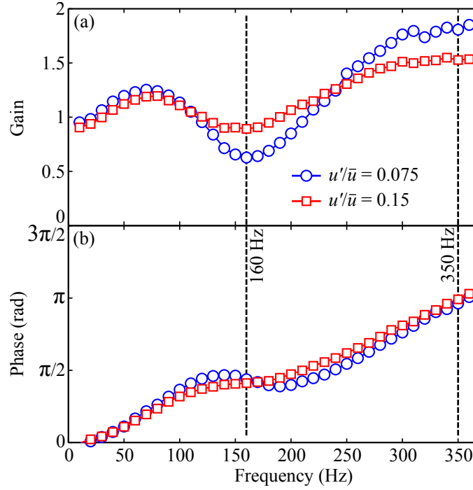
Figure 6.3: Flame transfer functions deduced from hot wire and PMT measurements for the flame at X_{H_2}^{fuel} = 0.60 , \phi = 0.70 , and U = 14 \text{ m} \cdot \text{s}^{-1} and two different velocity perturbation levels: u'/\bar{u} = 0.075 (blue) and u'/\bar{u} = 0.15 (red).
