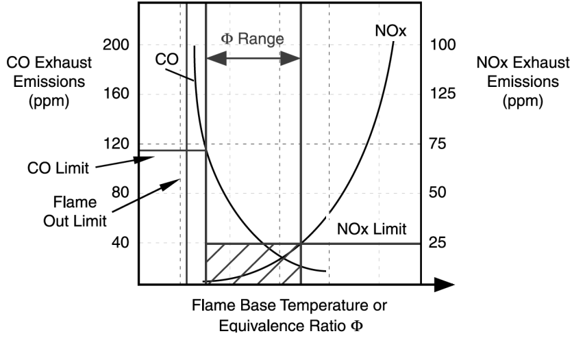
Figure 4: CO and NOx production from lean premixed combustion. Reproduced from Docquier and Candel (2002) . Adapted from Brown (1995) .
