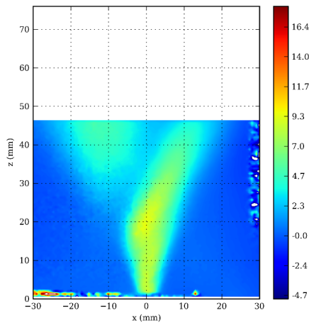
(e) PIV - U_z [m.s -1 ] - Plane Y = 7 mm
