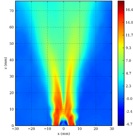
(b) LES - \widetilde{U}_z [m.s -1 ] - Plane Y = 0 mm
