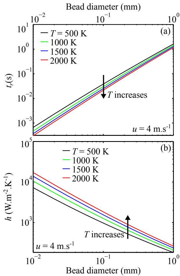
Figure 2.54: (a) Log/log plot of the evolution of the thermocouple response time t_r as a function of its bead diameter D at u = 4 \text{ m s}^{-1} and for different gas temperatures. (b) Evolution of the convective heat transfer coefficient h .
