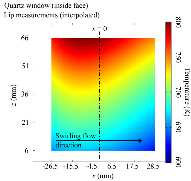
Figure 3.15: Top: Temperature, measured by LIP at the inner surface of a quartz window of the combustion chamber, of a \text{CH}_4/\text{H}_2/\text{air} flame at P = 4 kW, X_{\text{H}_2}^{\text{fuel}} = 0.60 , and \phi = 0.7 . Bottom: Linear interpolation of the data presented above.
