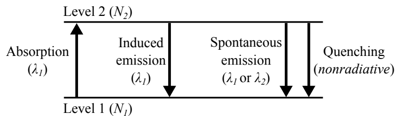
Figure 2.10: Schematic of the simplified two-level atom model for fluorescence. N_1 and N_2 stand for the populations of Levels 1 and 2. The wavelength of the photon emitted (or absorbed) is denoted by \lambda . Adapted from Daily (1997) .
