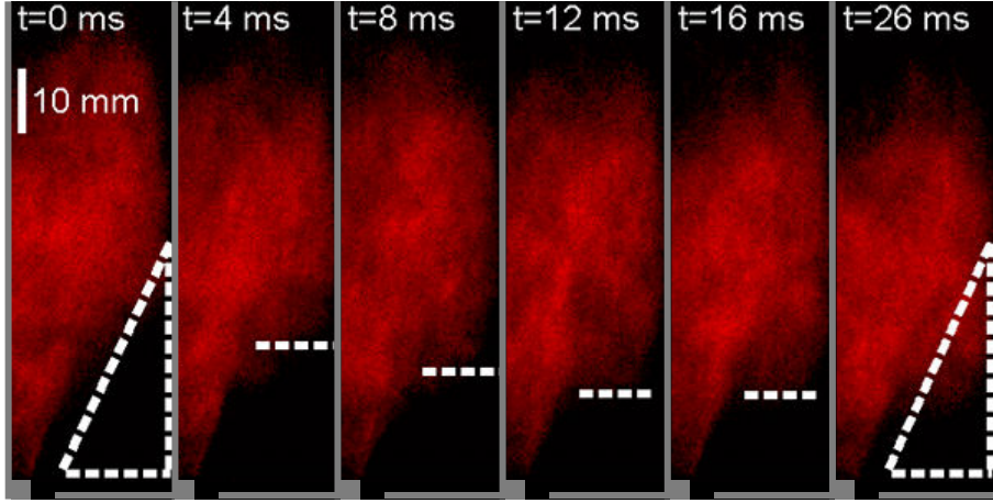
Figure 4.7: V to M shape transition captured with a high speed CMOS camera. The white triangle delineates approximately the ORZ boundaries and defines the interrogation zone used in Fig. 4.9. The left and right boundaries in these images respectively correspond to the burner axis and to the quartz tube wall. Swirl number S_5 = 0.40 , hydrogen enrichment X_{H_2}^{fuel} = 0.28 , bulk injection velocity U = 18 \text{ m} \cdot \text{s}^{-1} and equivalence ratio \phi = 0.54 . Injector set in configuration A.
