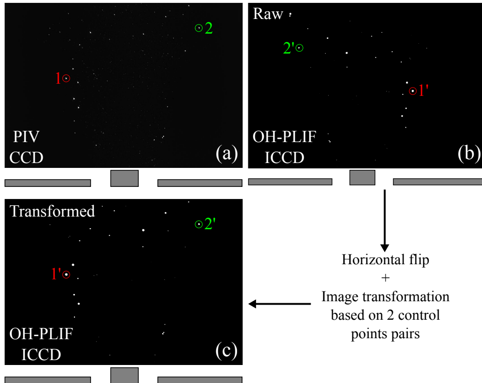
Figure 2.31: (a) Mie scattering image of ZrO_2 particles imaged onto the PIV CCD under non-reactive conditions. (b) Image of the same particles with the OH-PLIF ICCD at the same instant. (c) Corrected OH-PLIF image. See the electronic version of this document for a better image definition.
