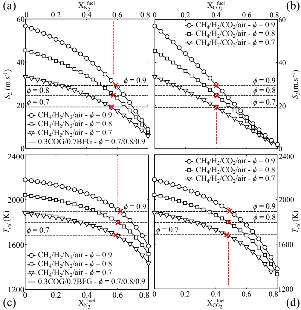
Figure 1.3: Laminar burning velocity S_L (a)-(b) and adiabatic flame temperature (c)-(d) of H_2/CH_4/N_2/air mixtures with X_{H_2}/(X_{H_2} + X_{CH_4}) = 0.60 when the molar fraction of N_2 (left column) and CO_2 (right column) in the fuel increases from X_{diluent}^{fuel} = 0 to 0.8. Results are shown for three different equivalence ratios \phi = 0.7, 0.8 , and 0.9. Values are superimposed to those found for 0.3COG/0.7BFG/air (molar fractions) mixtures at the same equivalence ratios. Red crosses show the diluent molar fraction in the fuel of the mixtures having the same laminar burning velocities or adiabatic flame temperature as the 0.3COG/0.7BFG/air mixture. The detailed chemistry mechanism from Lindstedt (1998) is used for calculations.
