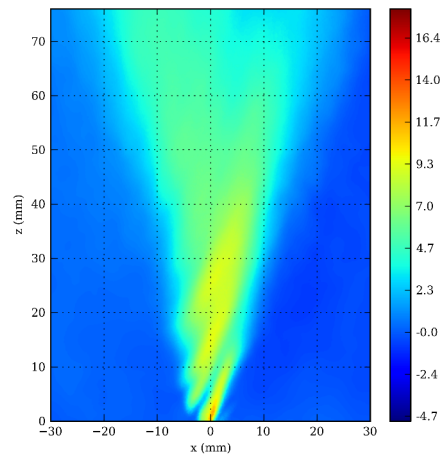
(f) LES - \widetilde{U}_z [m.s -1 ] - Plane Y = 7 mm
