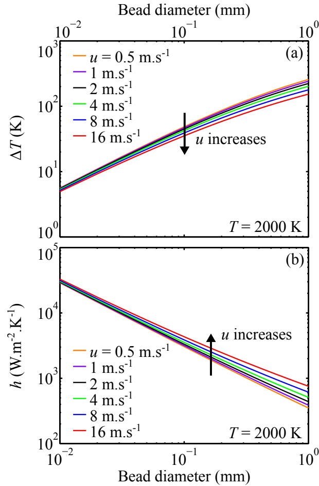
Figure 2.56: (a) Log/log plot of the evolution of the thermocouple temperature drop \Delta T as a function of its bead diameter D when the flow temperature is fixed to T = 2000 \text{ K} and for different gas velocities. (b) Evolution of the convective heat transfer coefficient h .
