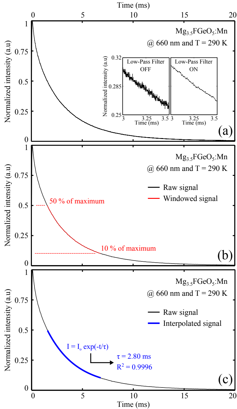
Figure 2.41: (a) Typical temporally decaying phosphorescent signal at 660 nm for Mg_{3.5}FGeO_5:Mn at T = 290\text{ K} . The effect of a low-pass filter applied to the signal is also visible. (b) A fraction of the raw signal is extracted to reduce interferences from the laser source and background light. The time window used for data reduction can be modified. (c) Exponential regression of the windowed signal and calculation of a decay time \tau and a coefficient of determination R^2 indicating the quality of the fit.
