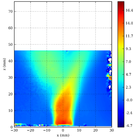
(c) PIV - U_z [m.s -1 ] - Plane Y = 4 mm
