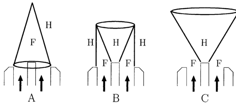
Figure 16: Shapes taken by a laminar flame above a burner depending on the location of the ignition point. Ignition is realized near the burner rim (B) or near the rod (C). Capital letters F and H respectively refer to fresh gases and hot burnt gases. Reproduced from Schuller et al. (2003).
